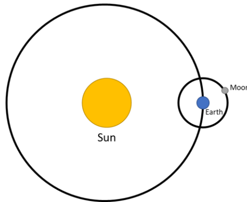
Figure 1. Bi-circular Four-Body Model (Spacecraft Not Shown)
