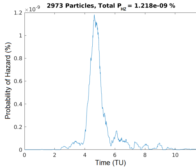
Figure 33. Statistics for Particles in Danger Zone: Mishap at L_2 , Spacecraft at L_1
