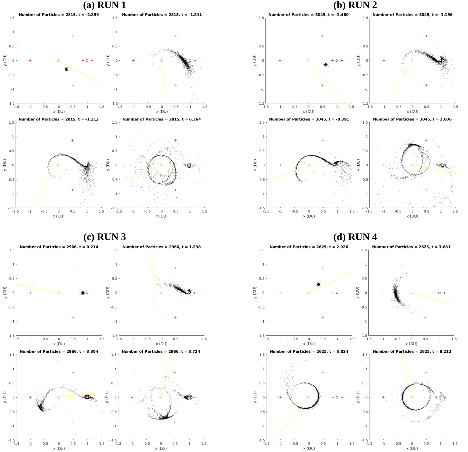
Figure 49. Snapshots of Selected Runs, Manifold Transfer Simulations: (a) Run 1; (b) Run 2; (c) Run 3; (d) Run 4
