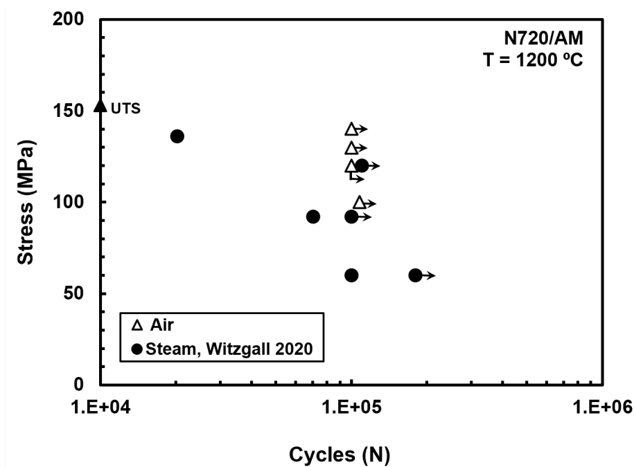
Figure 31. Fatigue S-N curves for Nextel™ 720/AM ceramic composite at 1200°C in air and in steam. Data in steam from Witzgall [27]. Arrow indicates that failure of specimen did not occur when the test was terminated.
