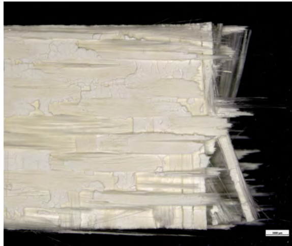
Figure 70. Optical micrograph of a N720/AM specimen fracture surface tested in tension-tension fatigue at 1200°C in air. \sigma_{\max} = 140 MPa, N_f > 100,000
