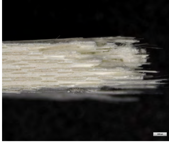
Figure 61. Optical micrograph of a N720/AM specimen fracture surface tested in tension-tension fatigue at 1200°C in air. \sigma_{\max} = 130 MPa, N_f > 100,000
