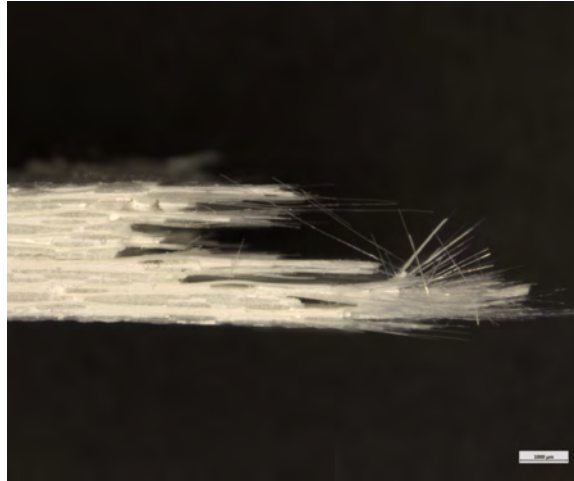
Figure 90. Optical micrograph of a N720/A specimen fracture surface tested in tension-tension fatigue at 1200°C in steam. \sigma_{\max} = 150 MPa, N_f = 700
