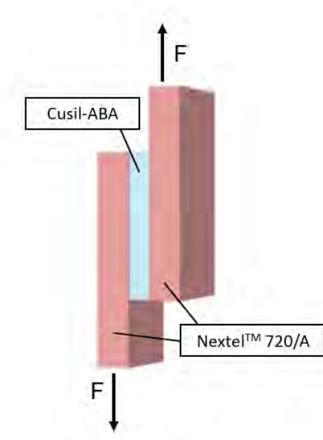
Figure 8. Schematic of joined specimens
