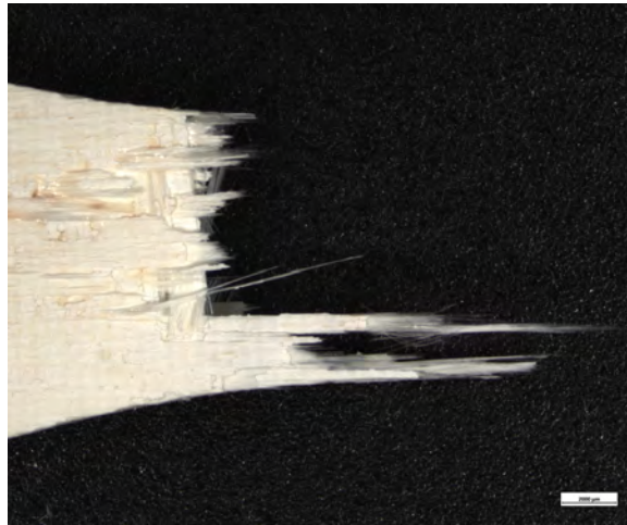
Figure 58. Optical micrograph of a N720/AM specimen fracture surface tested in tension-tension fatigue at 1200°C in air. \sigma_{\max} = 130 MPa, N_f > 100,000
