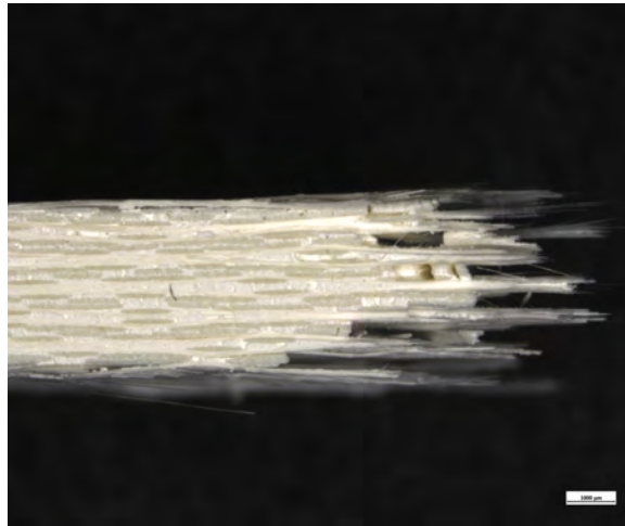
Figure 37. Optical micrograph of the fracture surface of N720/AM specimen tested in tension-tension fatigue at 1200°C in air. \sigma_{\max} = 100 MPa, N_f > 100000 .
