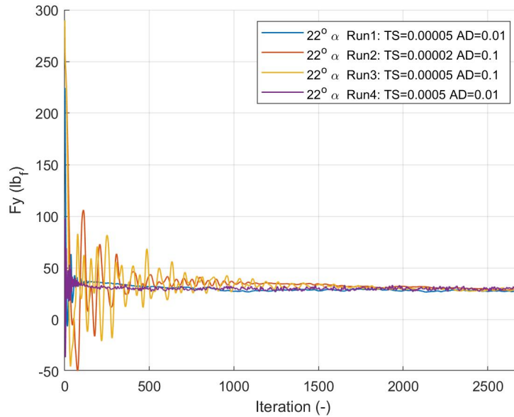
Figure 63. NACA 0012 Cropped Delta-Wing Baseline CFD Model Normal Force ( F_y ) Time Resolution Results, \alpha = 22^\circ , Re = 5 \times 10^5 , Time Step (TS) and Advective Damping (AD)
