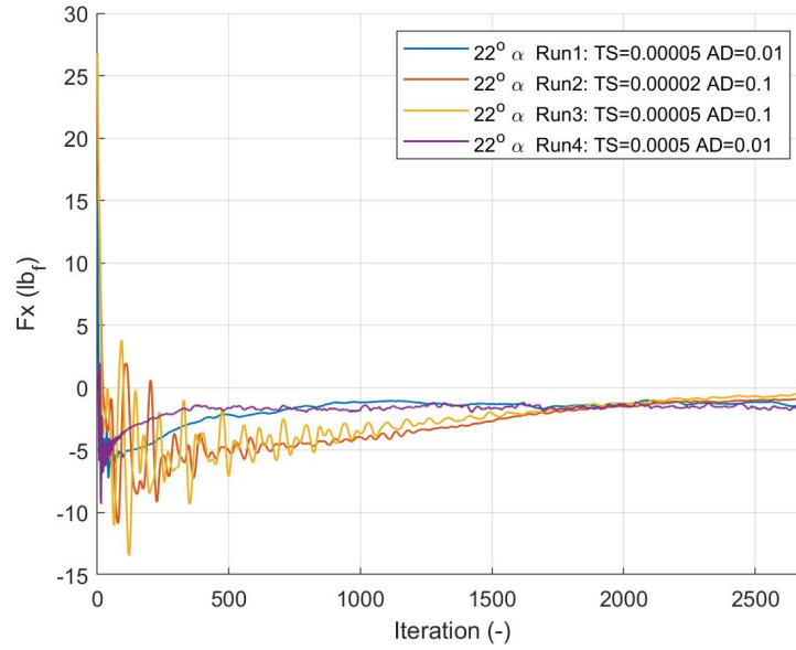
Figure 62. NACA 0012 Cropped Delta-Wing Baseline CFD Model Axial Force ( F_x ) Time Resolution Results, \alpha = 22^\circ , Re = 5 \times 10^5 , Time Step (TS) and Advective Damping (AD)
