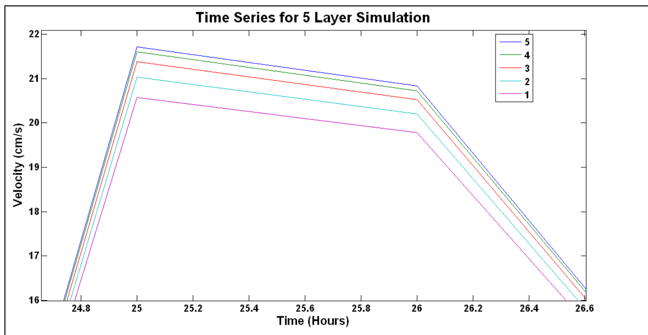
Figure 9. Vertical Velocity Distribution Time Series, Cell 44.
