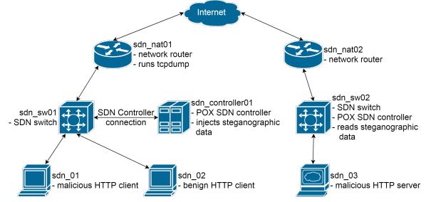
Figure 7: Experimental test-bed.
