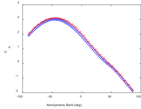
b) Normal Force
