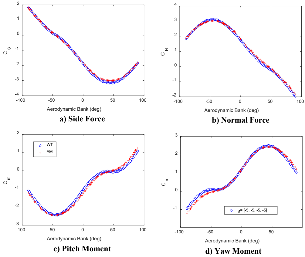
Fig. 13 Sample comparison between wind tunnel (WT) and aero model (AM), in body frame, roll sweep, AoA = 12°, Mach = 0.7, \delta = [-5 \ -5 \ -5 \ -5]
