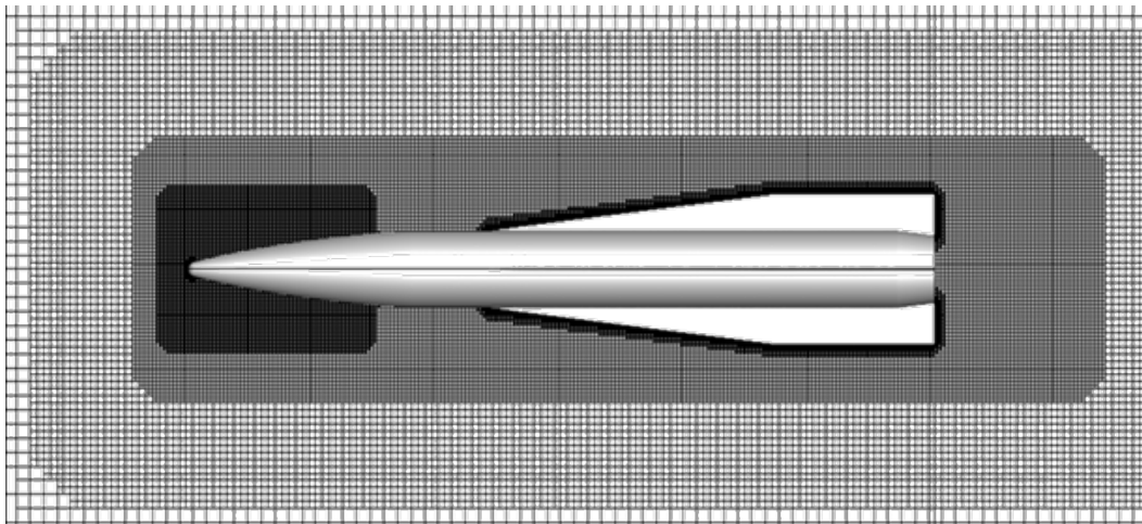
Fig. 2 Example Cart3D mesh
