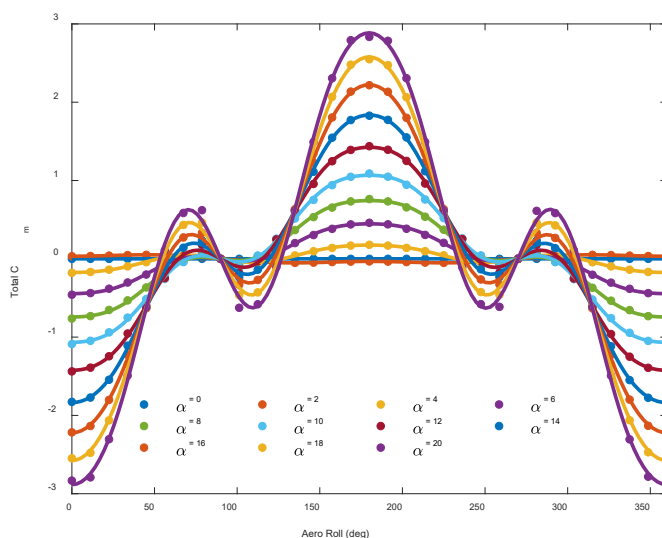
Fig. 6 Rigid aero surfaces, pitch moment CFD data at Mach 2 (dots). Fourier interpolation is superimposed (solid lines) showing smoothing, symmetry, and null points at \phi=90^\circ, 270^\circ .
