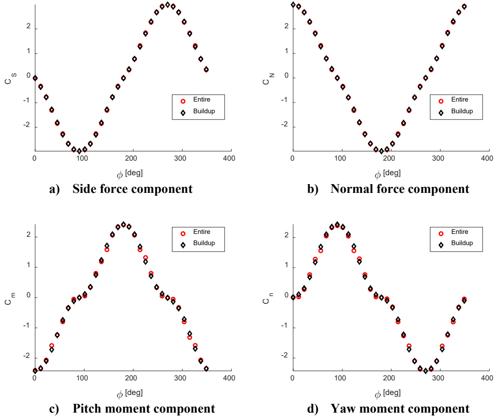
Fig. 9 Validating the superposition buildup. Sample results at \text{Mach} = 0.75 , \alpha = 12^\circ . Red circles are taken directly from CFD. Black diamonds show the total after applying the polynomial model for each component, then totaling in the body frame.
