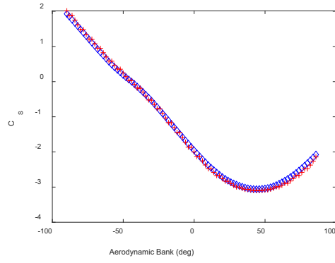
a) Side Force
