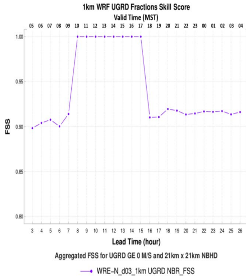
Fig. A-1 FSS, CSI, FBIAS, O-Rate, and F-Rate for 1-km WRF for UGRD GE 0 m/s
