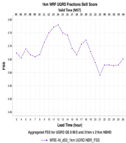
Fig. A-2 FSS, CSI, FBIAS, O-Rate, and F-Rate for 1-km WRF for UGRD GE 8 m/s
