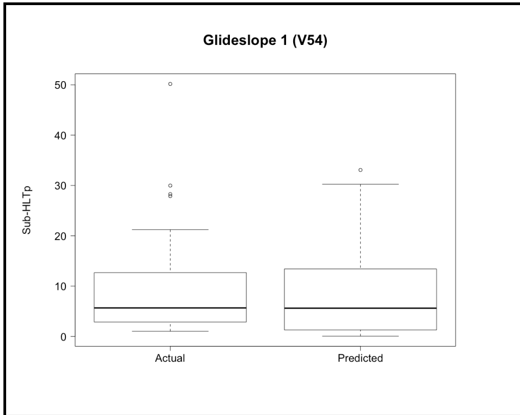
Figure 81. Glideslope 1 Actual vs. Predicted Scores Boxplot
