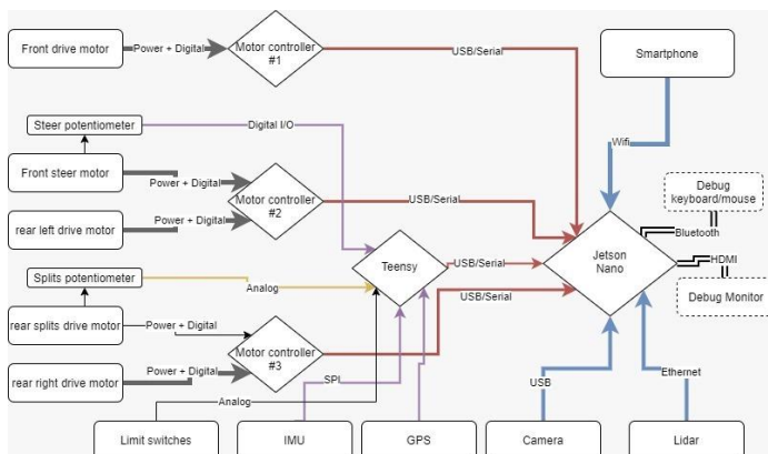
Figure 21: Control System Overview
