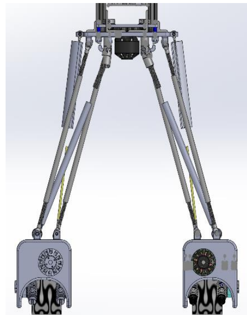
Figure 11. Variable Geometry Mechanism driven by Motors and Dual Linear Actuators
