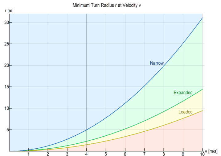
Figure 17: Minimum Required Turn Radius for Safe Turning Maneuvers
