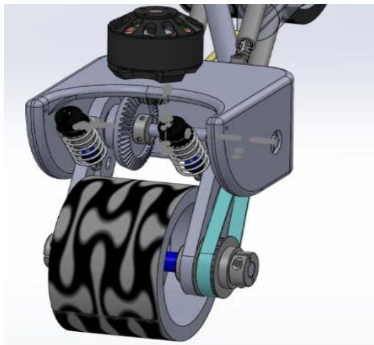
Figure 10. Rear Wheel Assembly with Suspension
