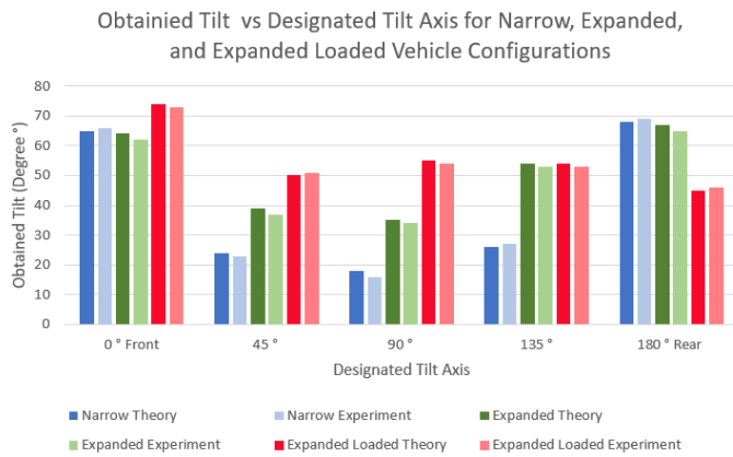
Chart 1: Tilt Orientation vs. Obtained Tilt Degree for Narrow, Expanded, and Expanded Loaded Configurations
