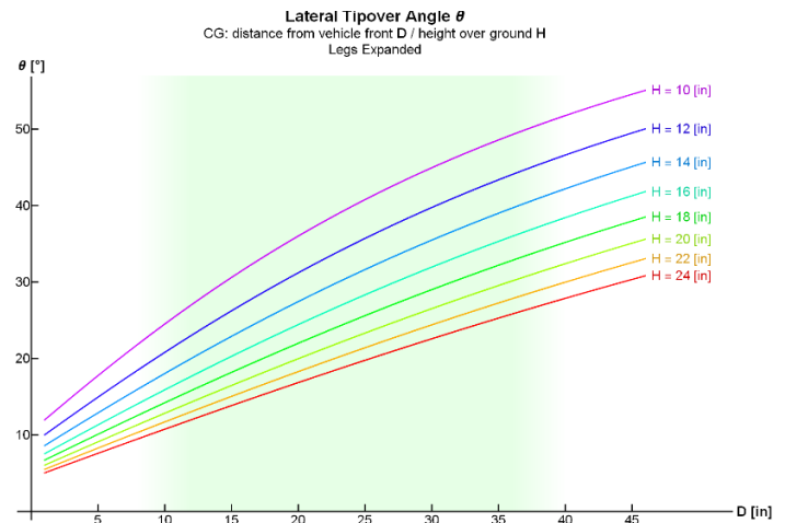
Figure 19: Lateral Tip over Angle Theta in terms of Distance D from Vehicle front over ground Height H Legs Expanded
