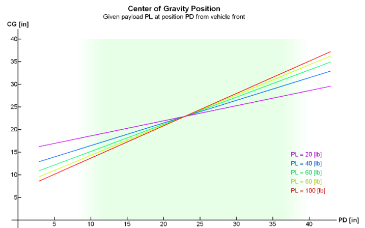
Figure 20: Center of Gravity Position given Payload PL at Position PD from Vehicle Front
