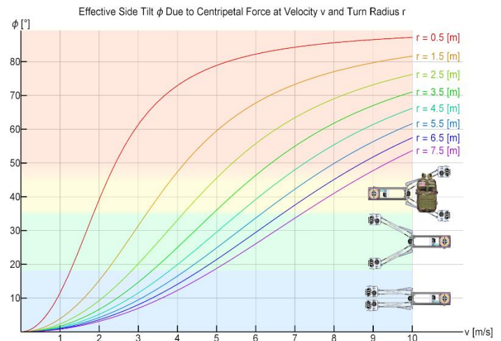
Figure 16: Effective Side Tilt Experienced During Turning Maneuvers
