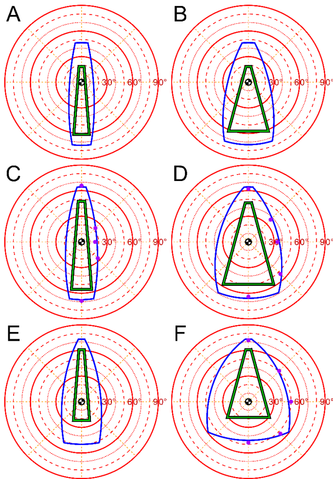
Figure 14: Six Vehicle Loading Configurations
