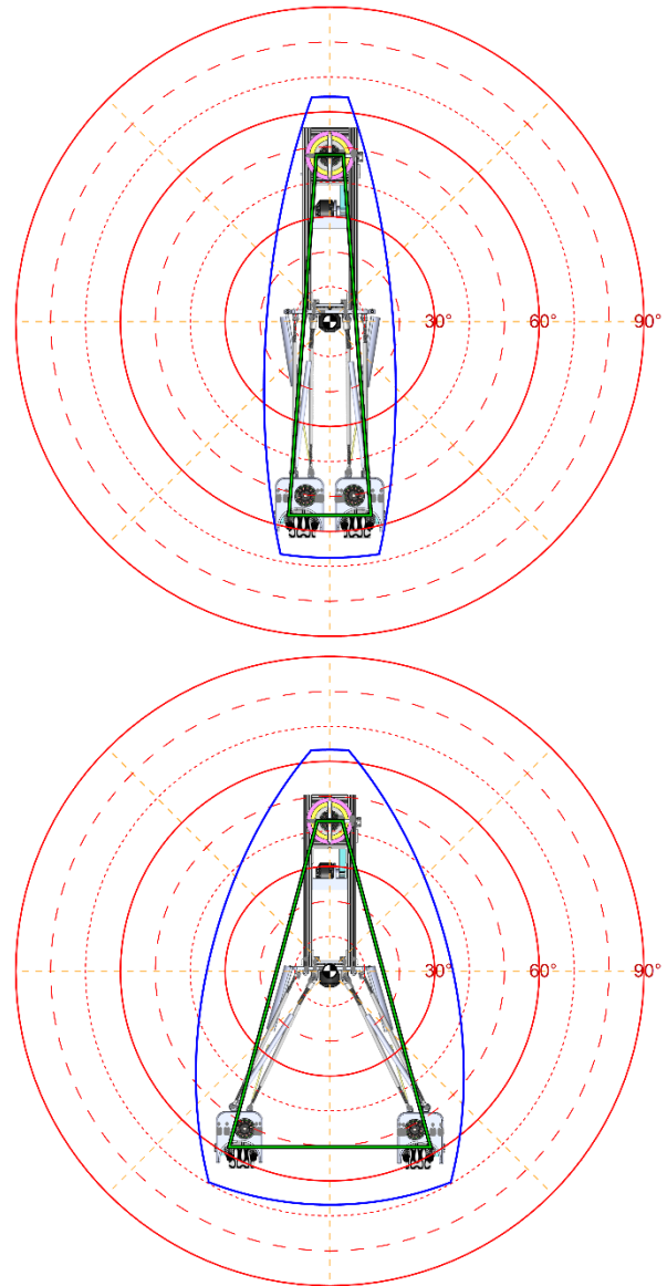
Figure 13: Stability plots of baseline Narrow and Expanded Unloaded Configurations with Vehicle Overlay
