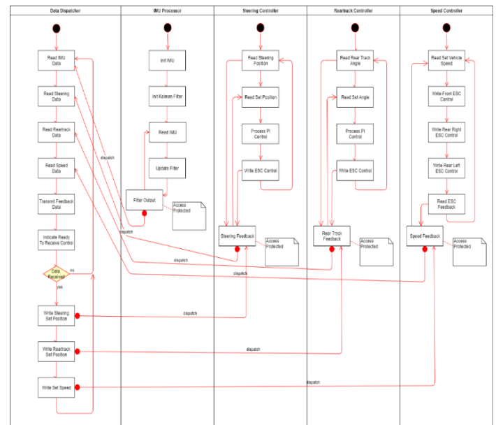
Figure 22: Control System
