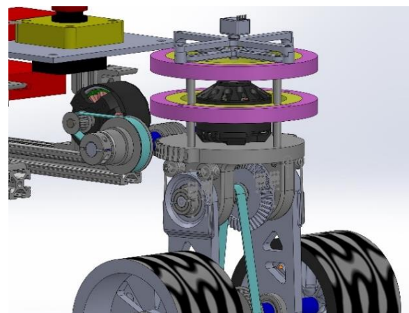
Figure 8. Front Steering Assembly
