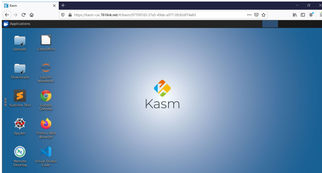
Fig. 1 Kasm desktop
