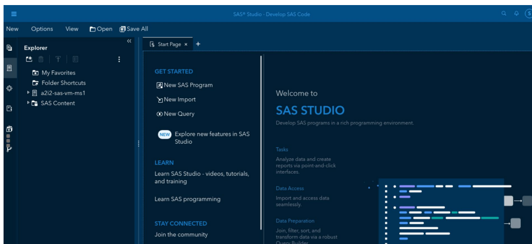
Fig. 3 SAS studio
