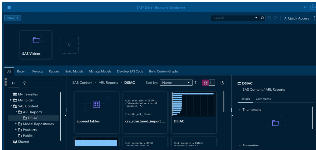
Fig. 2 SAS drive
