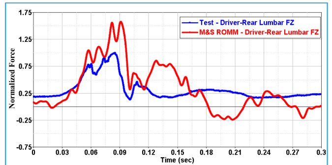
Figure 27: Driver Rear Lumbar FZ
