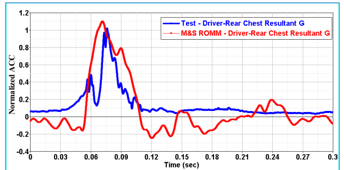
Figure 26: Driver Rear Chest Resultant Acceleration
