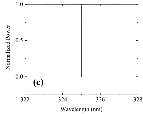
Figure 17. Normalized power of a WGM resonator confirming resonance at 325 nm. (a) Resonance when the WGM resonator has a Q-factor of 10^3 . (b) Resonance when the WGM resonator has a Q-factor of 10^4 . (c) Resonance when the WGM resonator has a Q-factor of 10^5 . Each increase in the Q-Factor decreases the FWHM.
