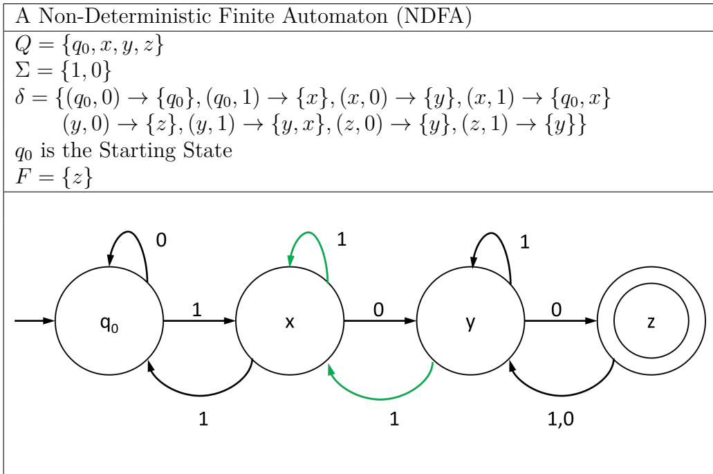
Figure 5. A N DFA created by adding two additional transitions (shown in green) to the FA in Figure 4 making multiple transitions for a given input possible from those corresponding states. This N DFA accepts the language 0^*1^+01^*(10)^*(01)^*(00)^*0
