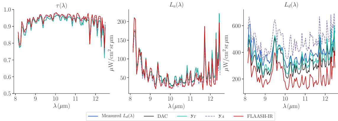
Figure 61. Applying MDAC to a collected data cube results in the two TUD predictions y_A and y_T shown. The \tau(\lambda) and L_d(\lambda) estimates are comparable for all methods. As expected, the largest model discrepancy is in the downwelling estimate, which relies on the selection of reflective pixels to estimate this term. This cube was collected at 1856L from an altitude of 0.45 km under clear sky conditions.
