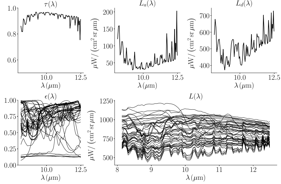
Figure 44. An example of set \mathbf{X} is shown in the bottom right plot where N = 50 . The lowest atmospheric temperature measurement was 296 K for the given TUD vector. The emissivity threshold, \varepsilon_t was 0.85, sampled P_E was 0.75, resulting in a mean emissivity less than 0.75 for 25% of the materials and a mean emissivity between 0.75 and 0.85 for 75% of the materials.
