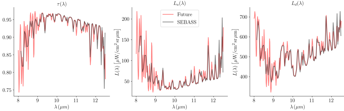
Figure 68. An example TUD vector is shown for the SEBASS sensor with 92 spectral bands and a future sensor using 256 spectral bands.
