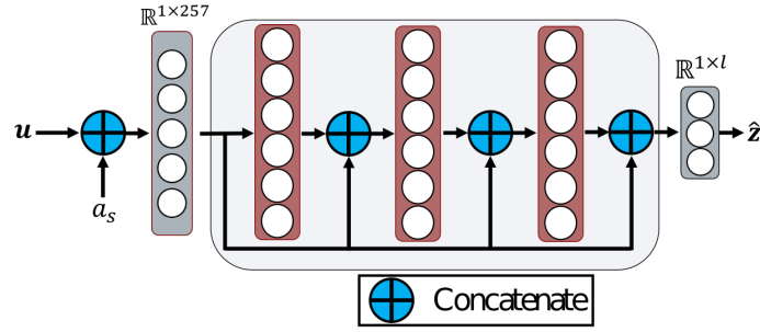
Figure 42. The \rho(\cdot) network is shown highlighting the use of skip connections to propagate the set representation to deeper layers. The input to this network is the result of the permutation-invariant set extraction concatenated with the sensor altitude, a_s . Each layer inside the network block contains 50 nodes and the predicted latent space contains 4 components.
