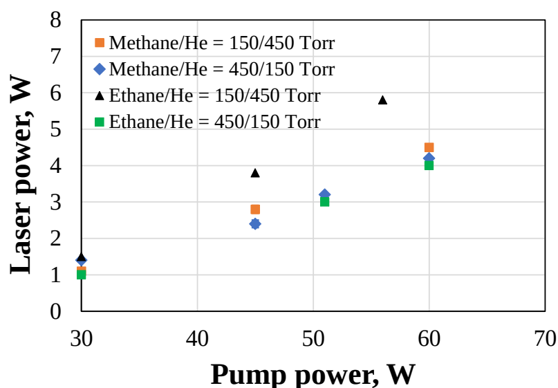
Fig. 2. Measured output laser power as a function of pump power in Cs static DPAL with different compositions of the buffer gas.
