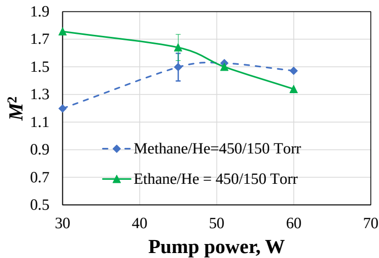
Fig.4. Measured beam quality factor M^2 as a function of pump power in Cs static DPAL with high molar fractions of methane and ethane in the buffer gas.
