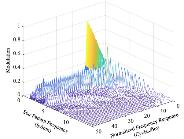
Fig. 11. FSD graph of a single 2D projection image.
