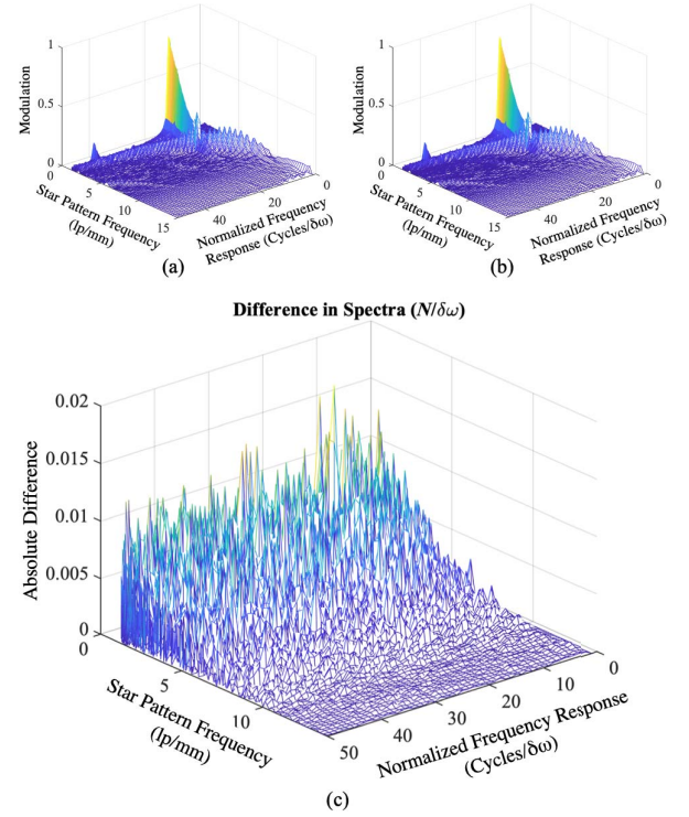
Fig. 10. Sampling rates: (a) 512, (b) 2048, and their difference (c) used to determine optimal sampling for the FSD.
