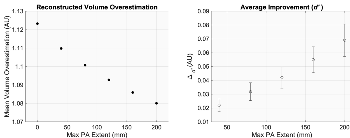
Figure 8: Mean volume overestimation as a function of PA source motion (left). Improvement in d' for bowtie acquisition geometries with PA-source motion ranging from 40 mm to 200 mm (right).
