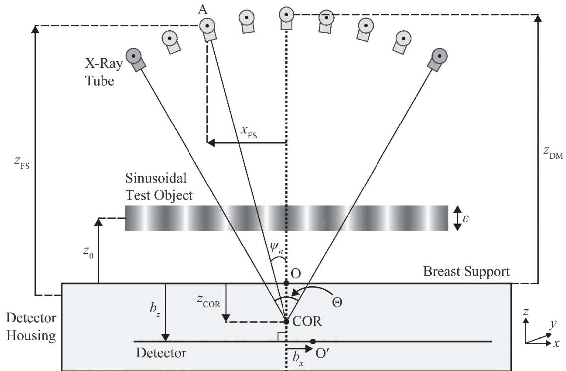
Figure 4. Diagram of source motion in a circular arc. The origin (O) is the midpoint of the chest-wall side of the breast support. The primed origin (O') is the corresponding midpoint of the detector. The test object is a thin rectangular strip with a sinusoidal attenuation coefficient.
