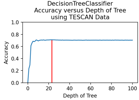
Figure 6. Accuracy versus depth of tree trained on TESCOAN data. The red line shows where the maximum accuracy was achieved.
