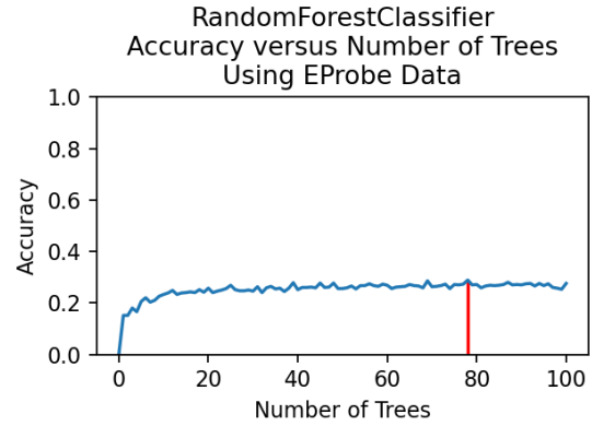
Figure 9. Accuracy versus number of trees for a Random Forest classifier trained on EProbe data.
