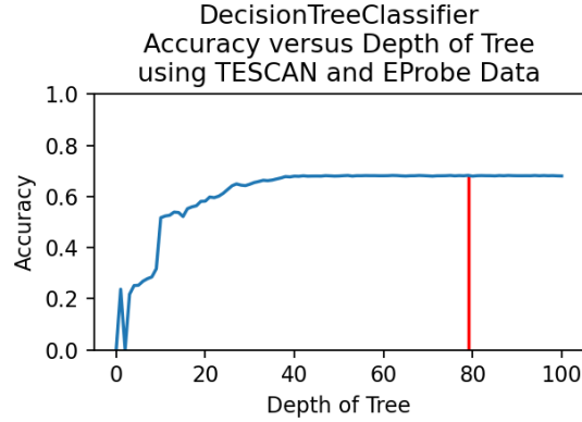
Figure 7. Accuracy versus depth of tree trained on both TESCOAN and EProbe data. The red line shows where the maximum accuracy was achieved.
