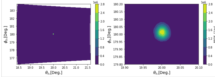
Figure 4.8: Contour plot (and a zoomed in plot) of the BRDF of the lab mirror illuminated at \theta_i=20^\circ in scatter coordinate space. The mirror appears to be highly specular and isotropic at first glance. This is because the sample appears very similar to the simulated data generated in scatter space, where a “small circle” was generated by the contour plots.
