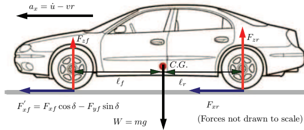
Fig. 3 Longitudinal load transfer force distribution.
