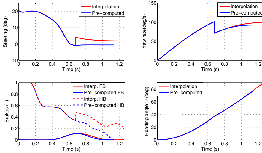
Fig. 11 State evolution comparison under disturbance.
