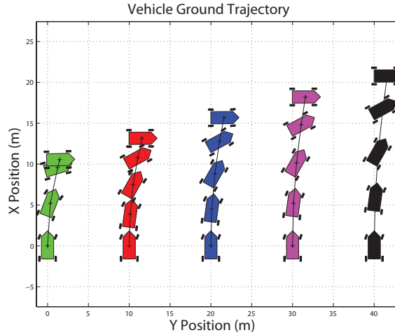
Fig. 5 Pre-computed solutions for different initial vehicle velocities (dry asphalt case, corresponding to \mu = 0.8 ).
