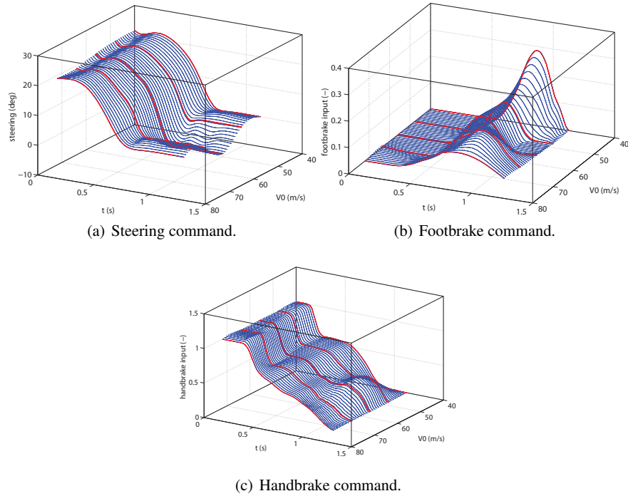
Fig. 9 Interpolated optimal control histories.
