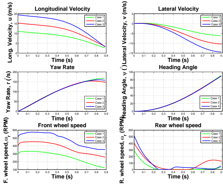
Fig. 8 Optimal open-loop state trajectories generated with GPOPS.
