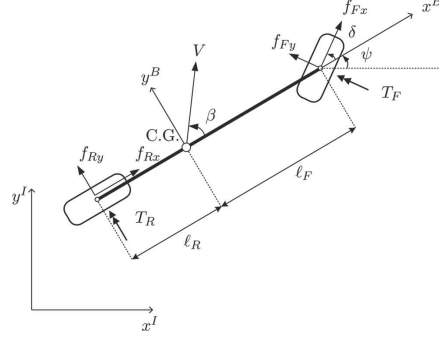
Fig. 2 Schematic of bicycle model.
