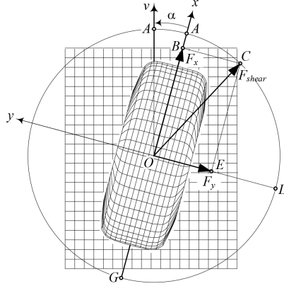
Fig. 4 The friction circle concept (from [18]).
