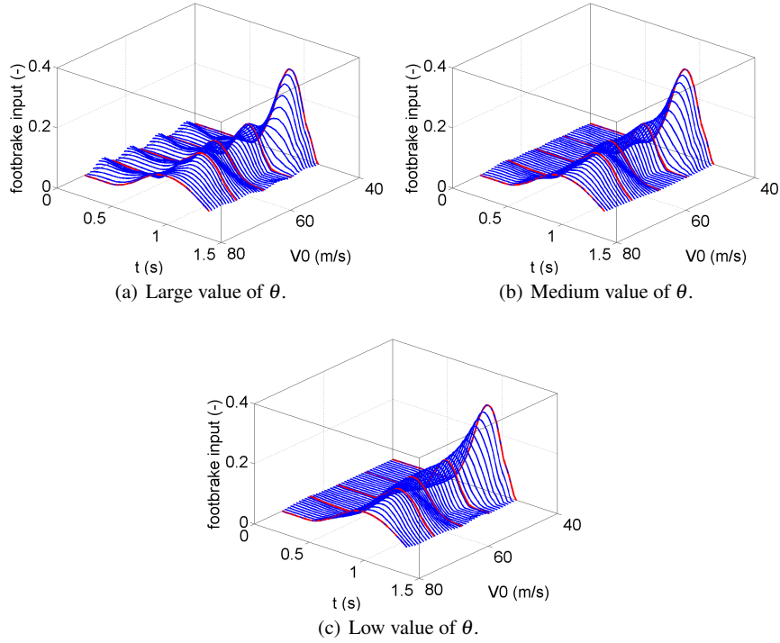
Fig. 10 Effect of correlation parameter \theta on the optimal footbrake command response surface.
