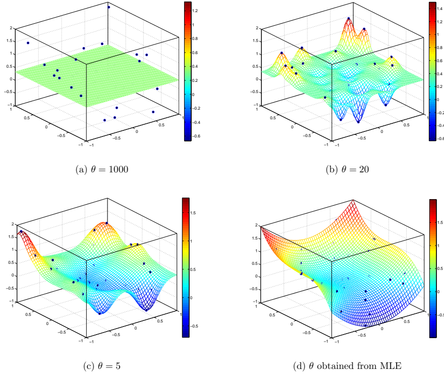
Fig. 6 Influence of the parameter \theta in the response surface.
