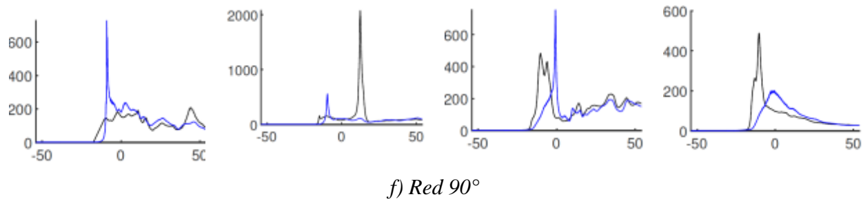
Figure 30: Turbulence intensities across landing spots #2, #4, #7 and #8 (in that order from the left) for various WOD directions; black line corresponds to z = 3 m while blue line corresponds to z = 6 m; “green” winds are from the starboard side of the ship and “red” winds from the portside [41]
