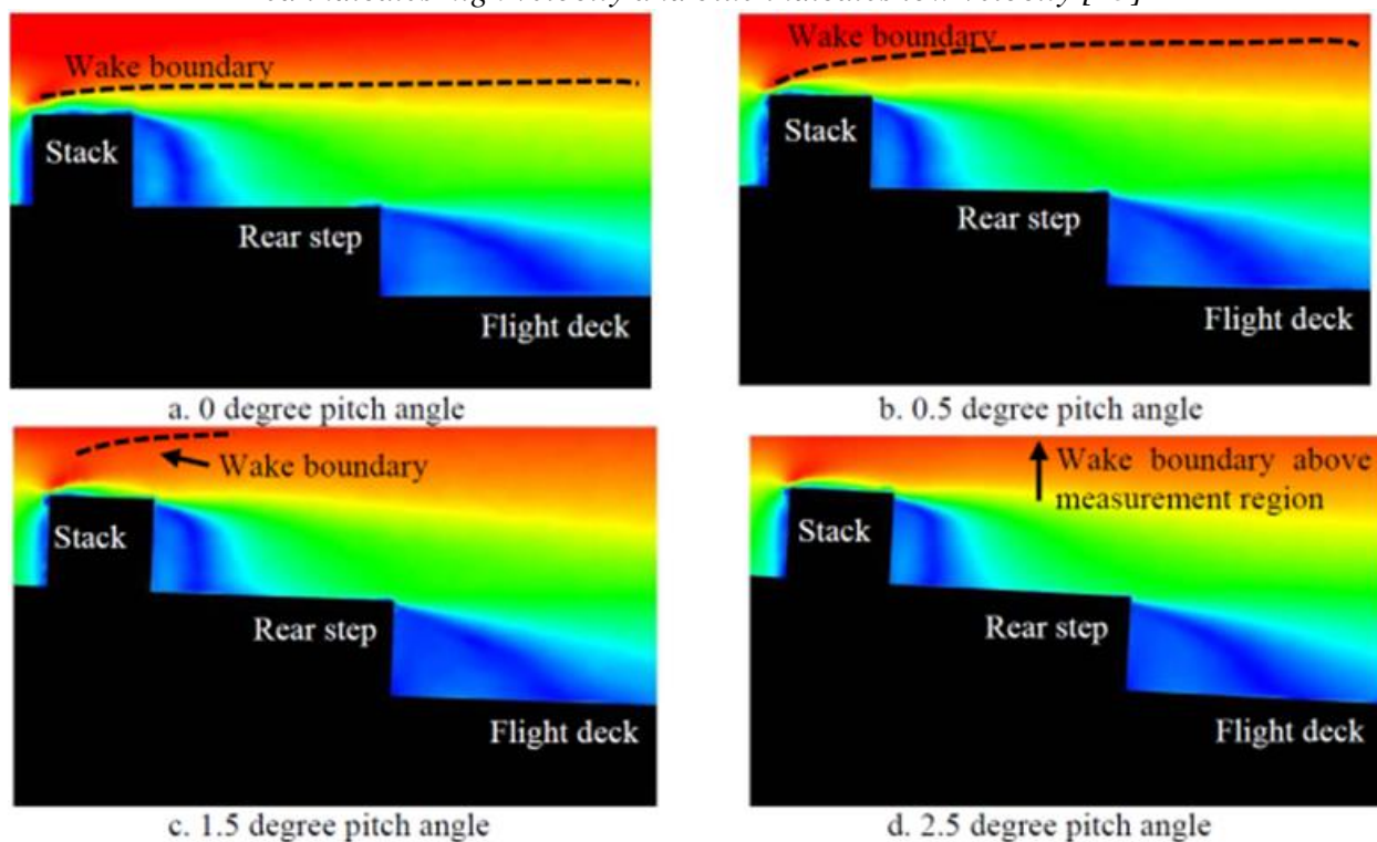
Figure 39: Effect of static pitch angle on mean velocity magnitude; red indicates high velocity and blue indicates low velocity [45]
