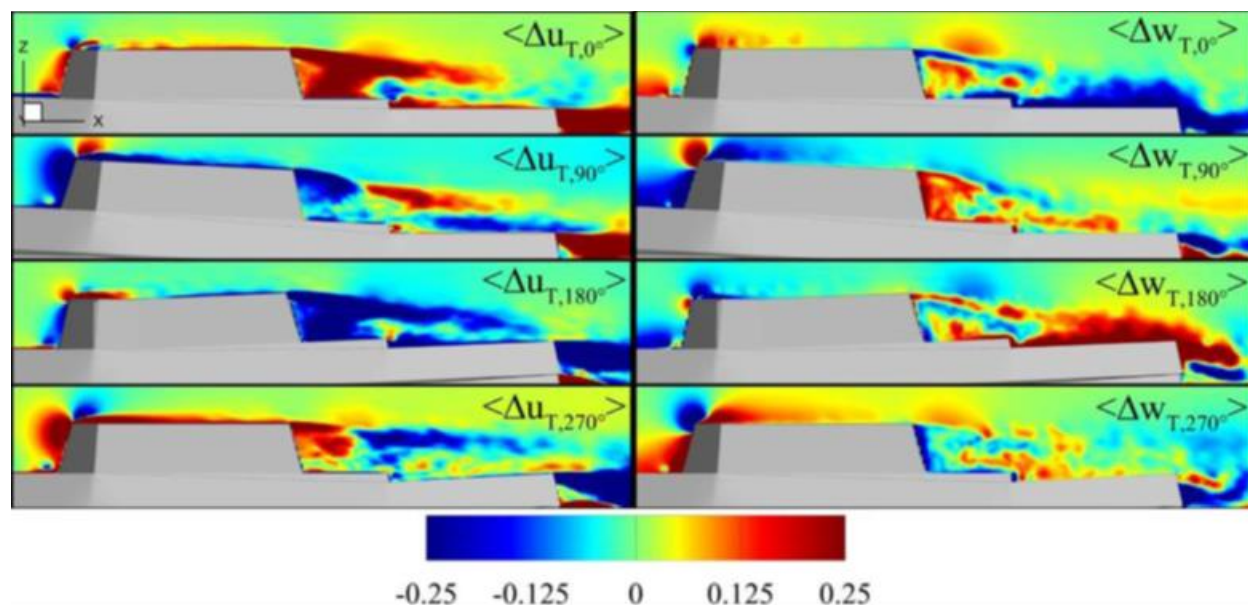
Figure 49: Phase-averaged deviations of longitudinal \Delta u_T (left) and vertical \Delta w_T (right) velocities from baseline over one wave cycle period; 0^\circ corresponds to the instance when the wave crest or peak is at the bow and the wave trough is at \lambda = 0.6 L , where \lambda is the wave length and L = 154 m is the ship model length; velocities are nondimensionalized using an arbitrary speed of U_0 = 25 kts [47]
