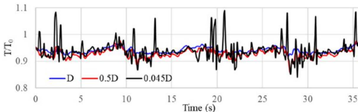
Figure 52: Instantaneous thrust produced by three scaled versions of a simplified SH-60 helicopter rotor model located 30 ft above the center of the flight deck of the ONRT ship advancing at 15 kts with a 35 kt headwind (SS6) during one-way coupled simulations [47]
