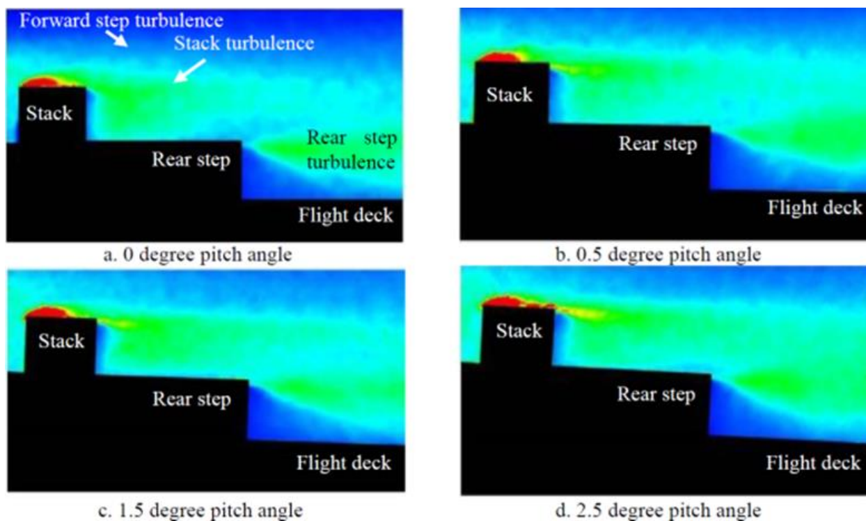
Figure 40: Effect of static pitch angle on TKE; red indicates high TKE and blue indicates low TKE [45]
