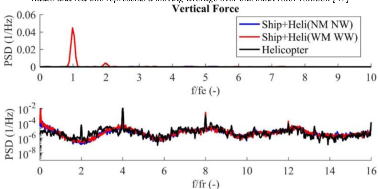
Figure 55: Frequency response functions corresponding to vertical force time-histories in Figure 54; f_e is the wave encounter frequency, and f_r is the main rotor rotational frequency [47]
