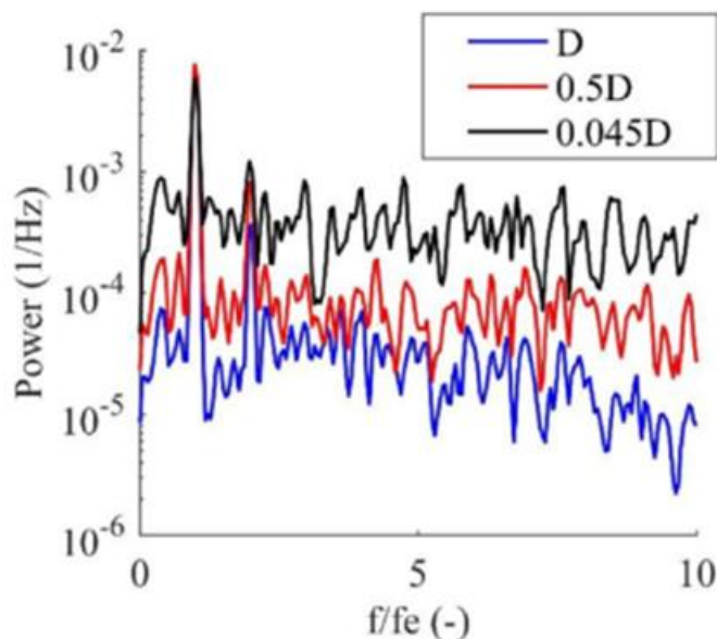
Figure 53: Frequency response function corresponding to thrust time-histories in Figure 52; f_e is the wave encounter frequency [47]
