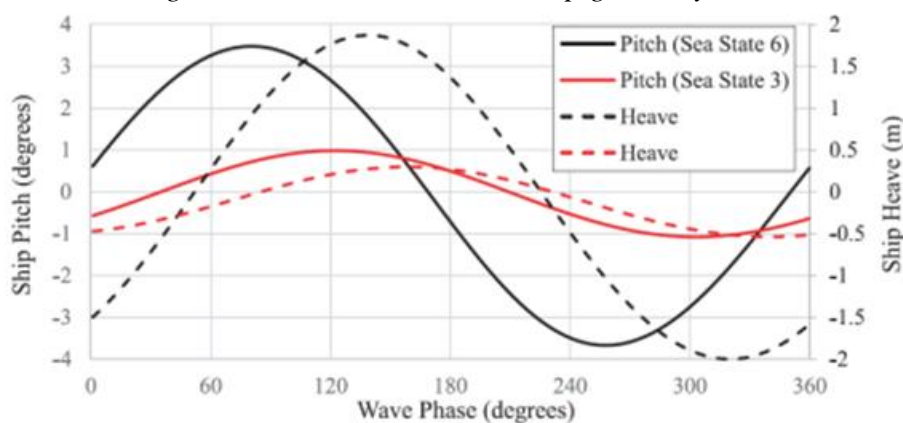
Figure 46: Ship pitch and heave motions through one wave encounter period for SS3 and SS6 [38]; 0^\circ corresponds to the instance when the wave crest or peak is at the bow and the wave trough is at \lambda = 0.6 L , where \lambda is the wave length and L = 154 m is the ship model length [47]
