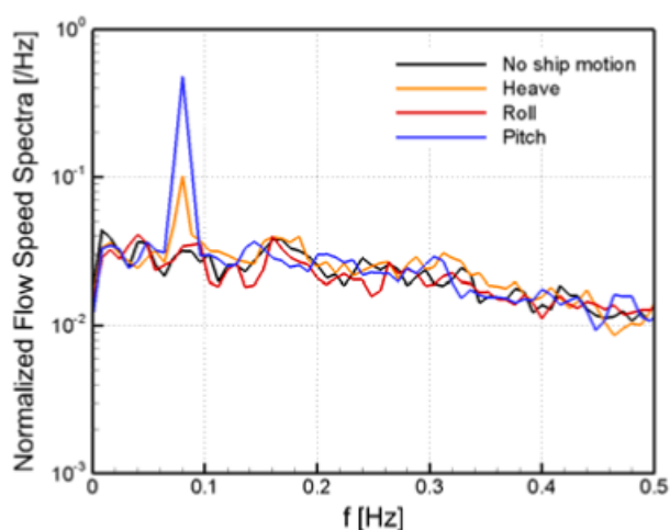
Figure 44: Spectrum of velocity magnitude measured by probe #3 from Figure 43(b) for isolated single DOF deck motion [46]
