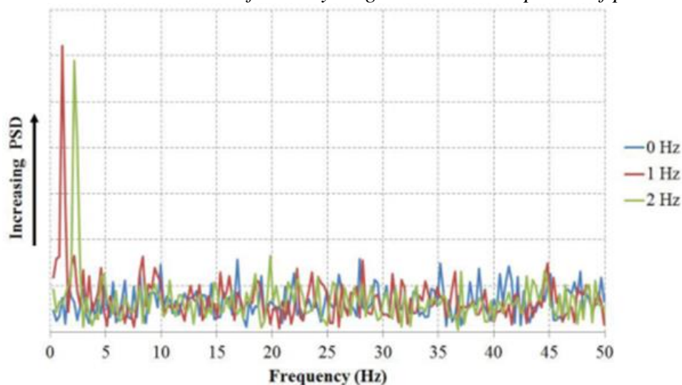
Figure 42: Spectrum of velocity magnitude at a point located horizontally at hangar and vertically at 1.4 times hangar height with ship oscillating in pitch attitude [45]
