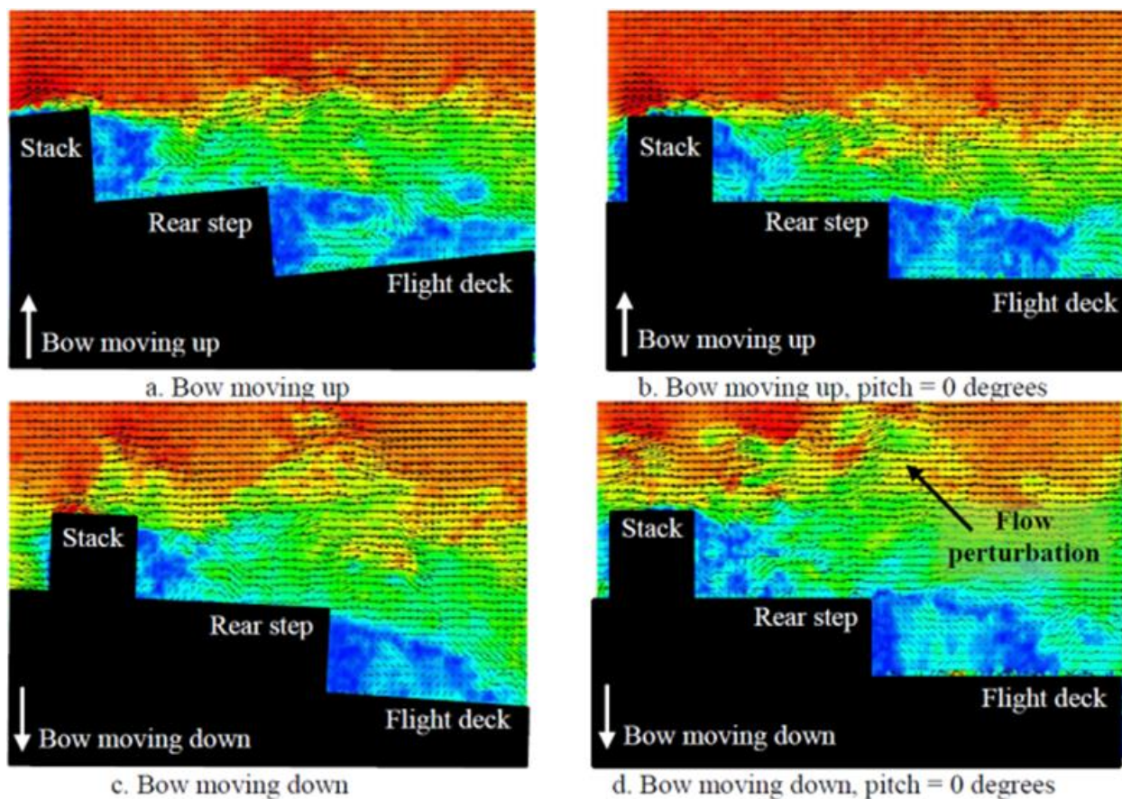
Figure 41: Instantaneous contours of velocity magnitude over one period of pitch motion [45]
