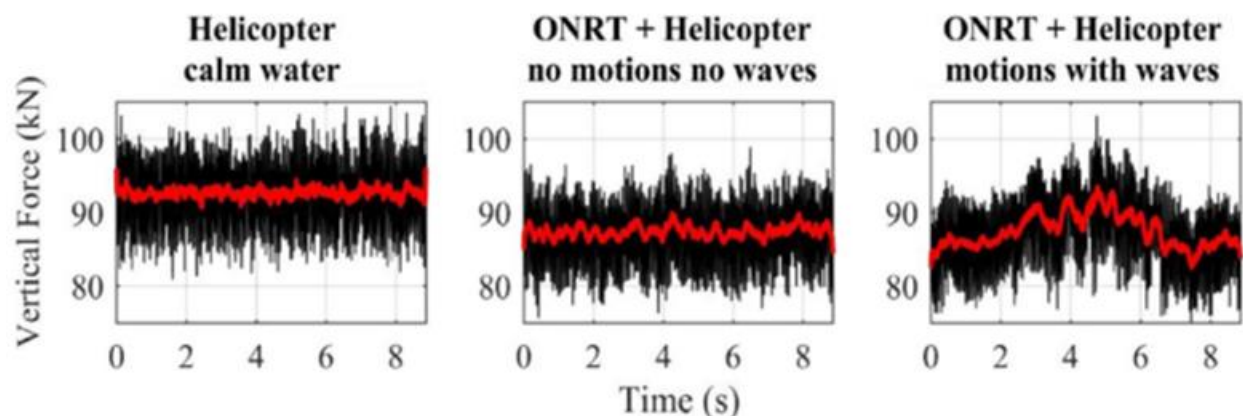
Figure 54: Time-histories of vertical force generated by a simplified SH-60 helicopter model located 30 ft above the center of the flight deck of the ONRT ship advancing at 15 kts with a 35 kt headwind (SS6) during two-way coupled simulations; black line indicates instantaneous values and red line represents a moving-average over one main rotor rotation [47]
