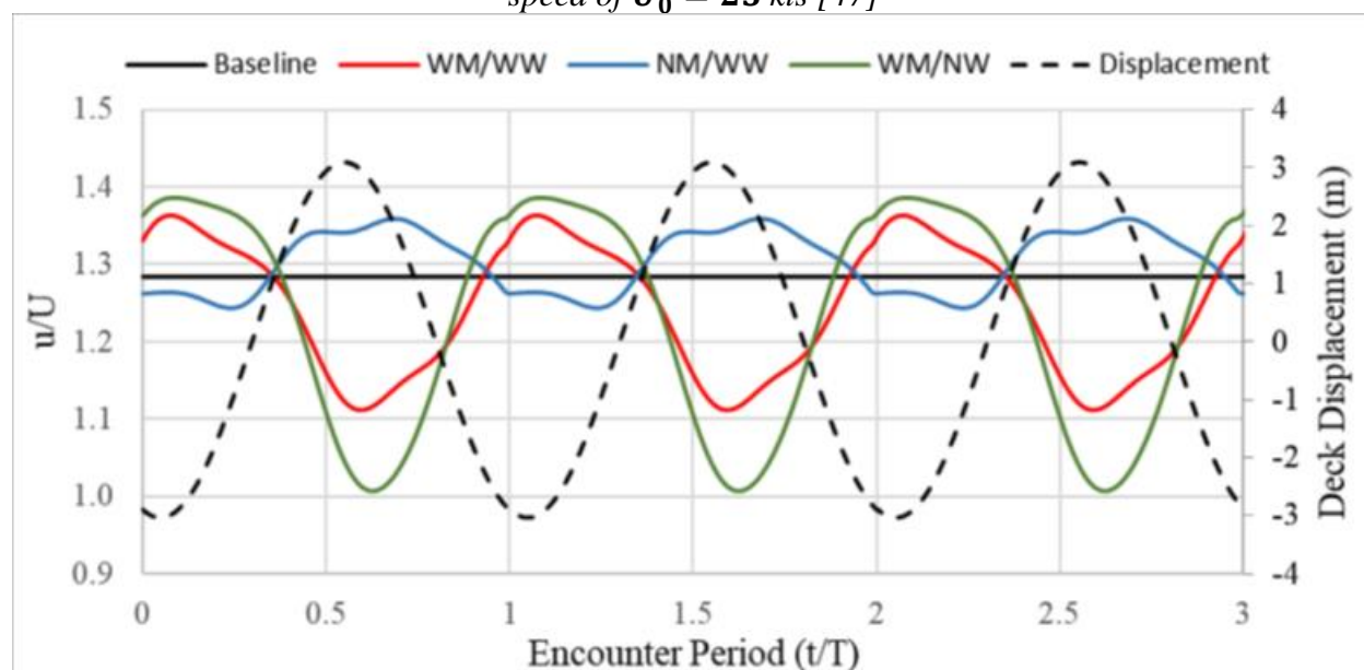
Figure 50: Phase-averaged longitudinal velocity at a point 30 ft above the center of the flight deck of ONRT advancing at 15 kts with a 35 kt headwind (SS6); wave encounter period is 8.5 s [47]
