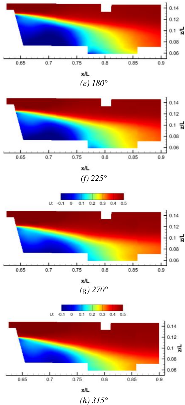
Figure 60: Mean longitudinal velocity contours for different phase angles of ship motion; velocity values are given in meters-per-second [48]
