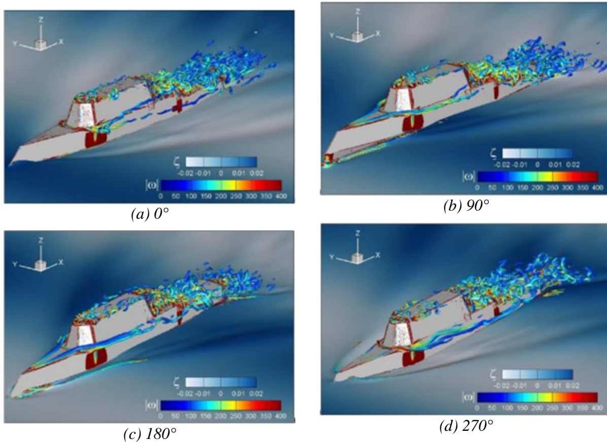
Figure 47: Isosurfaces of vortical structures for ONRT advancing at 15 kts in a 35 kts headwind (SS6) with wave and ship motion; 0^\circ corresponds to the instance when the wave crest or peak is at the bow and the wave trough is at \lambda = 0.6 L , where \lambda is the wave length and L = 154 m is the ship model length [47]
