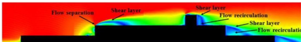
Figure 38: Time-averaged velocity magnitude over SFS2 model ship at even keel in a headwind; red indicates high velocity and blue indicates low velocity [45]
