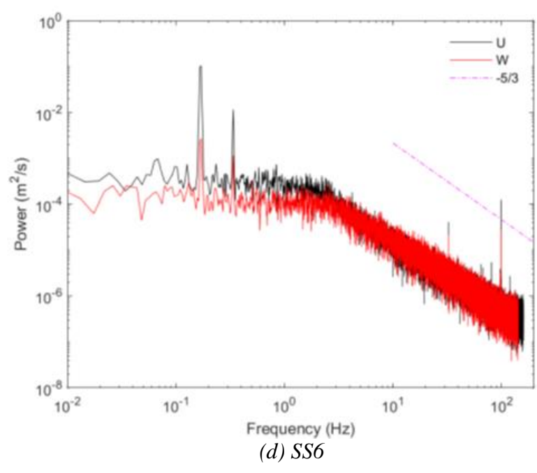
Figure 62: Frequency spectra of longitudinal and vertical velocities recorded at (x/L, z/L) = (0.888, 0.110) (see Figure 57) during water channel experiments [48]
