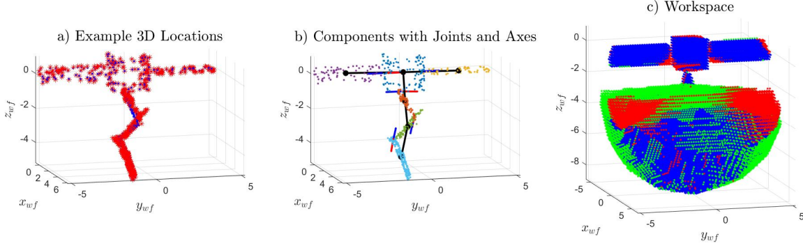
Figure 17. Results with trajectory matrix and inspection route noise. a) Truth (blue \cdot ) and calculated (red * ) 3D position of points for first frame. b) Calculated points, kinematic chain, joint locations, and axes (truth in blue calculated in red) for first frame. Points in each component are a different color. c) Grid positions in both true and calculated workspace (blue \cdot ), Grid positions in only true workspace (red \cdot ), Grid positions in only calculated workspace (green \cdot ).
