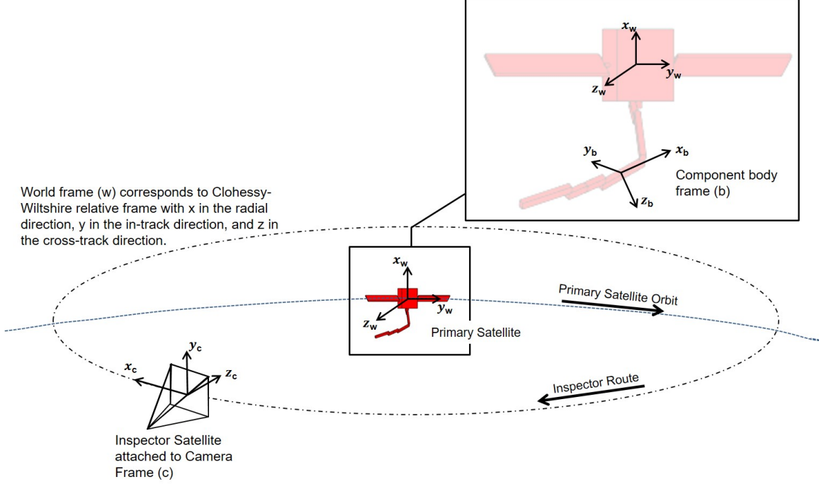
Figure 10. Reference frames used in this work. The ‘world frame’ ( w ) corresponds to the CW frame and moves with the primary satellite in its orbit. Each component has a ‘body frame’ ( b ) attached to it which is arbitrarily assigned. The ‘camera frame’ ( c ) is attached to the inspector camera with the positive z axis along the optical axis and the positive x axis aligned with the camera’s direction of travel in the world frame.
