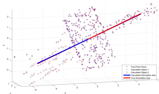
Figure 9. Point cloud and articulation axis results for a single trial.
