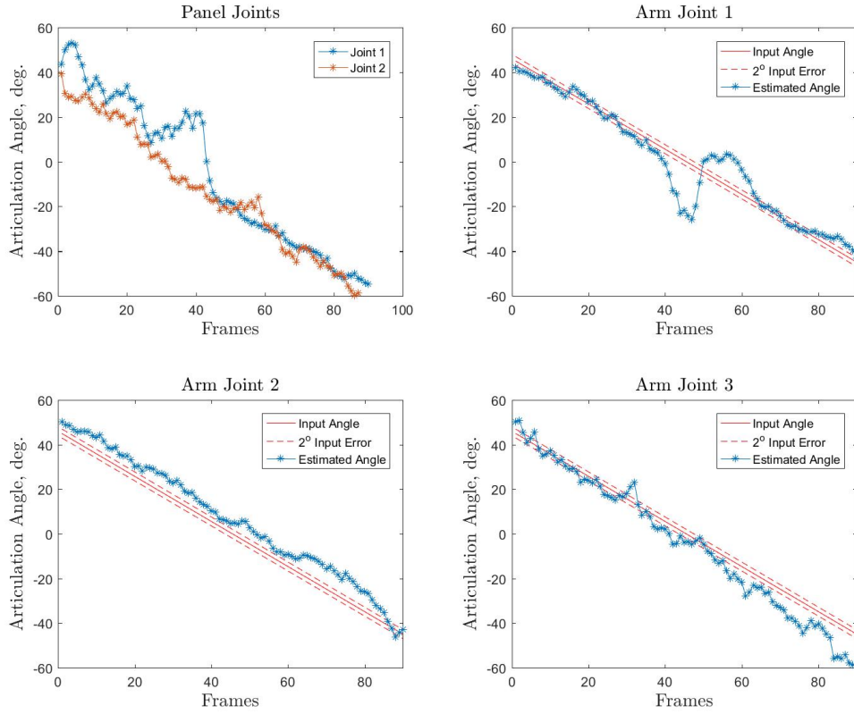
Figure 44. Estimated articulation angle results for all 5 joints. Panels input angles were not captured. Arm input angles were linear, however \pm 2^\circ input inaccuracy is likely
