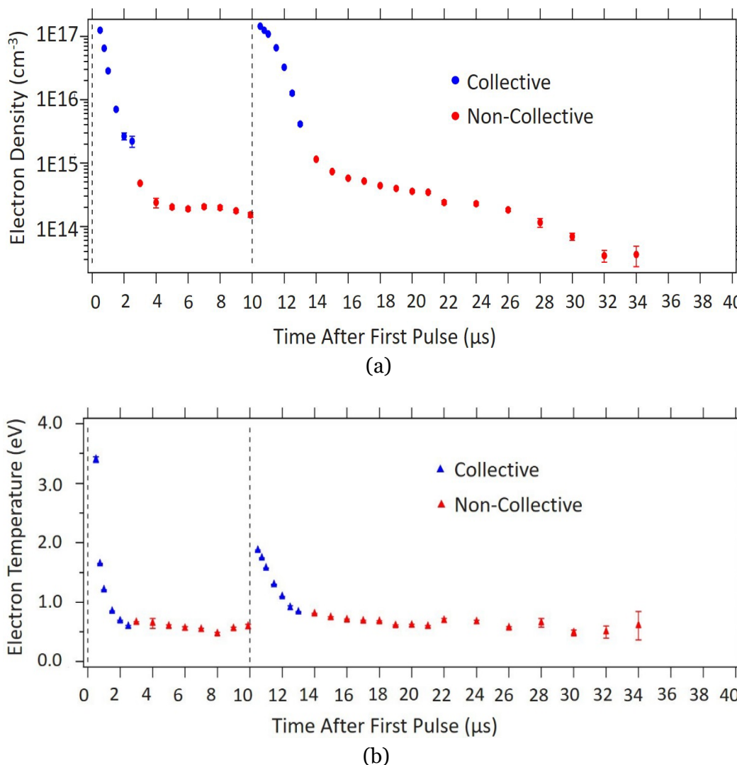
Figure 23: Electron density (a) and electron temperature (b) measurements with a burst of two pulse discharges at a 100 kHz repetition rate at various times after the initial pulse
