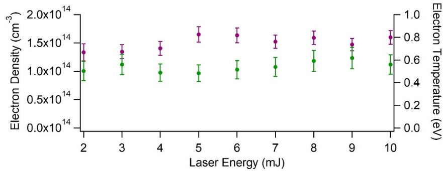
Figure 26: Laser power variation for non-collective scatter 10 \mu s after the discharge with electron density (purple) and electron temperature (green) measured
