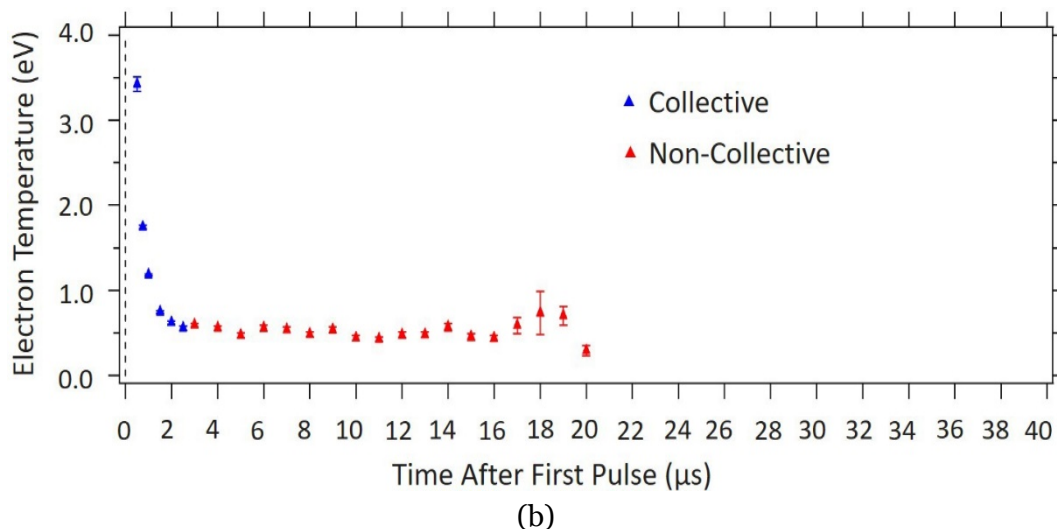
Figure 22: Electron density (a) and electron temperature (b) measurements of the single nanosecond pulse discharge at various times after the pulse.
