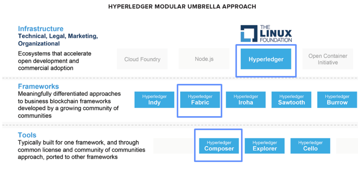
Figure 10: Hyperledger architecture.
