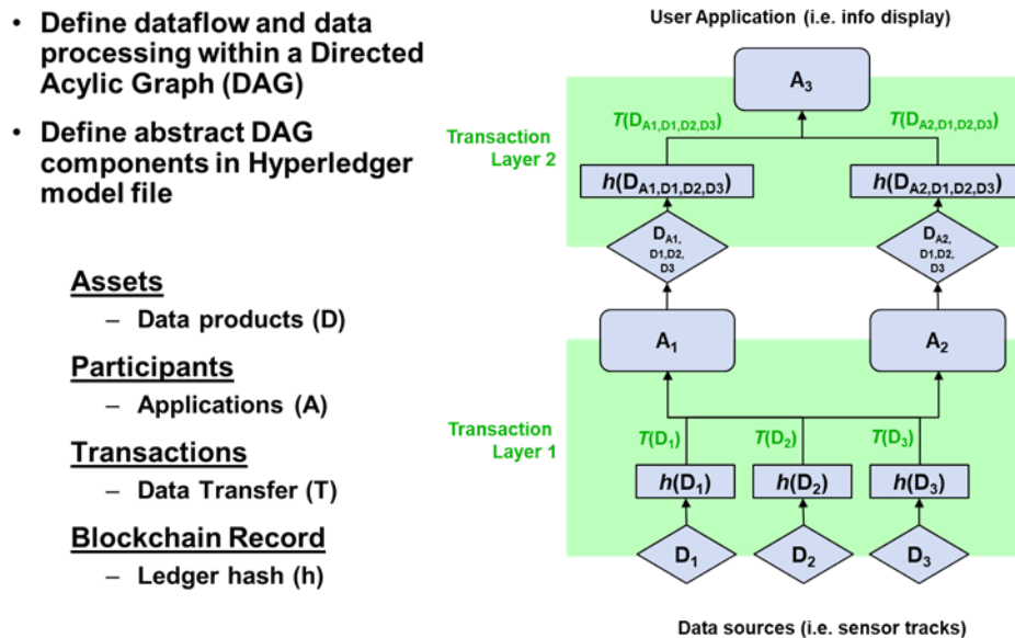
Figure 11: Mapping a processing system to a directed-acyclic-graph.
