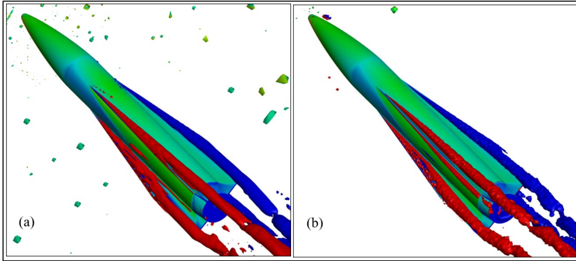
Fig. 22 Surface contours of pressure coefficient superimposed with iso-surfaces of scaled Q -criterion ( Q_s = 1.5 ) colored by streamwise vorticity at \phi = 45^\circ and computed by (a) Cart3D and (b) \text{CFD}^{++}
