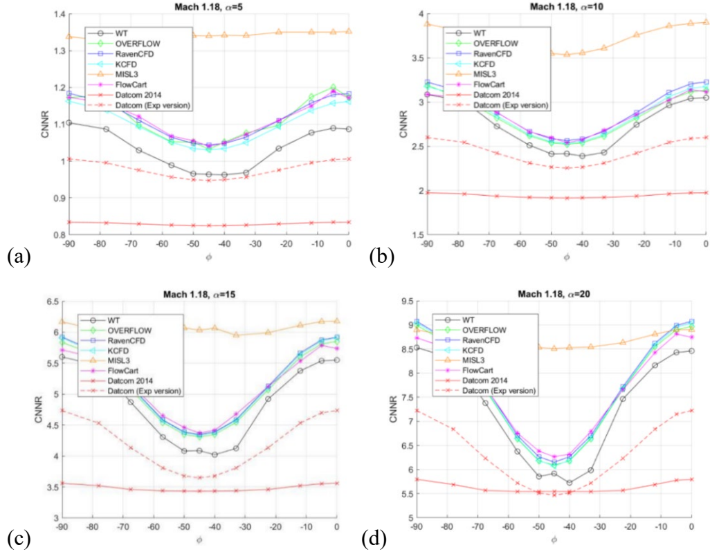
Fig. 10 C_{NNR} variation with roll angle from WT and aeroprediction codes for Configuration 1 at Mach 1.18 and \alpha = (a) 5°, (b) 10°, (c) 15°, and (d) 20°
