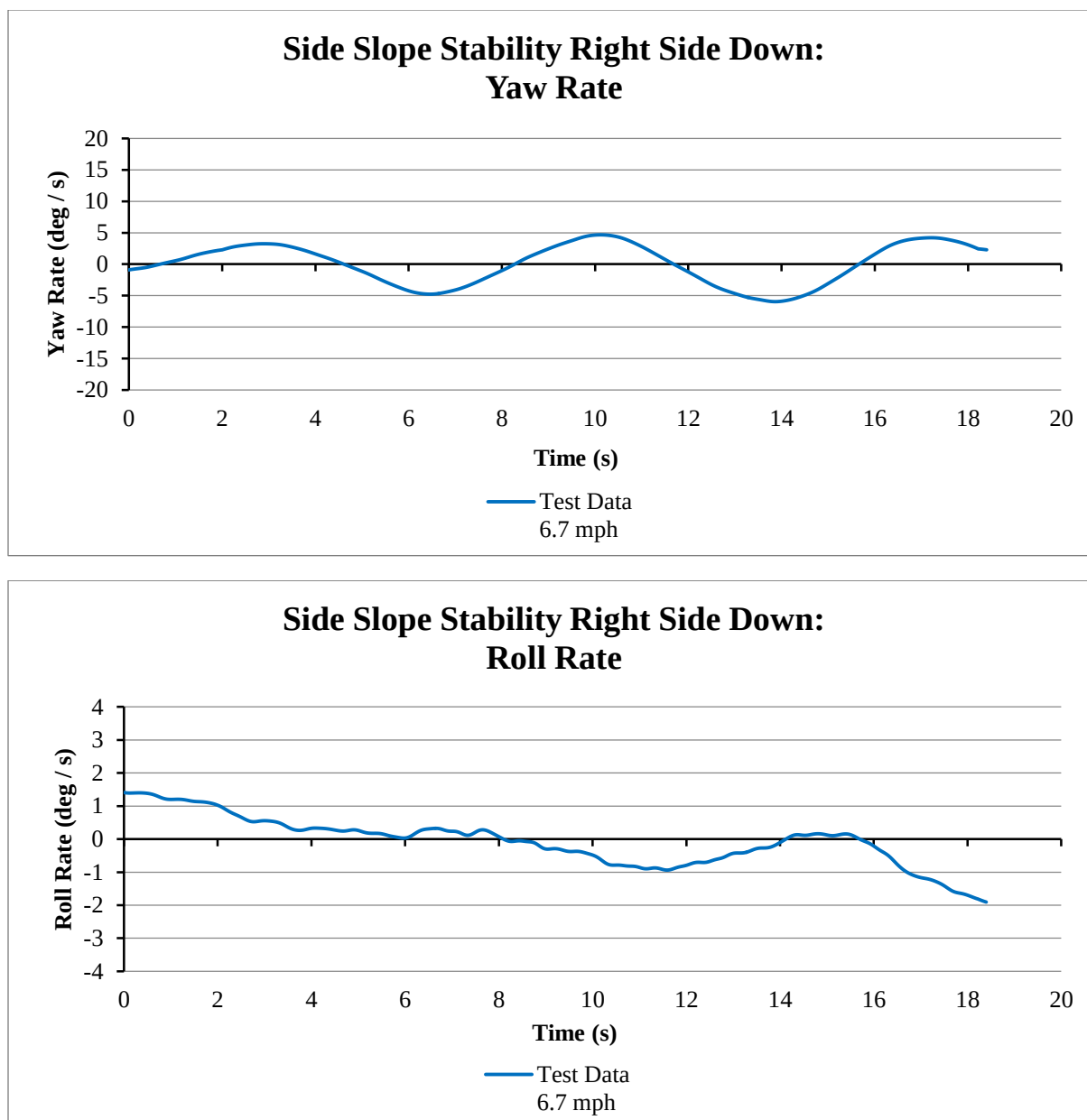
Figure G.14: Side Slope Stability Right Side Down, Yaw and Roll Rate on Compacted Soil (Non-deformable).
