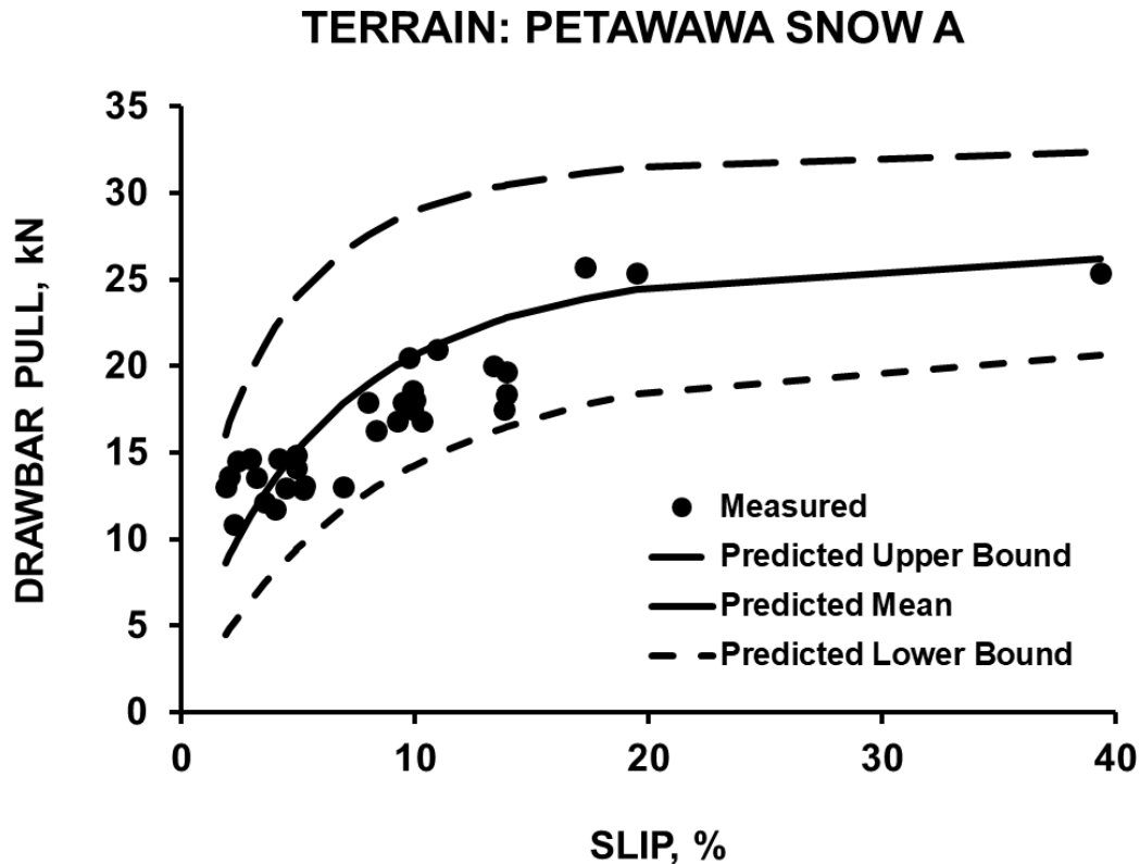
Figure F.5: Graphical Correlation between the Measured Drawbar Pull-slip Relationship of the APC (Test Vehicle) on Petawawa Snow A, together with that Predicted by NTPVM.
