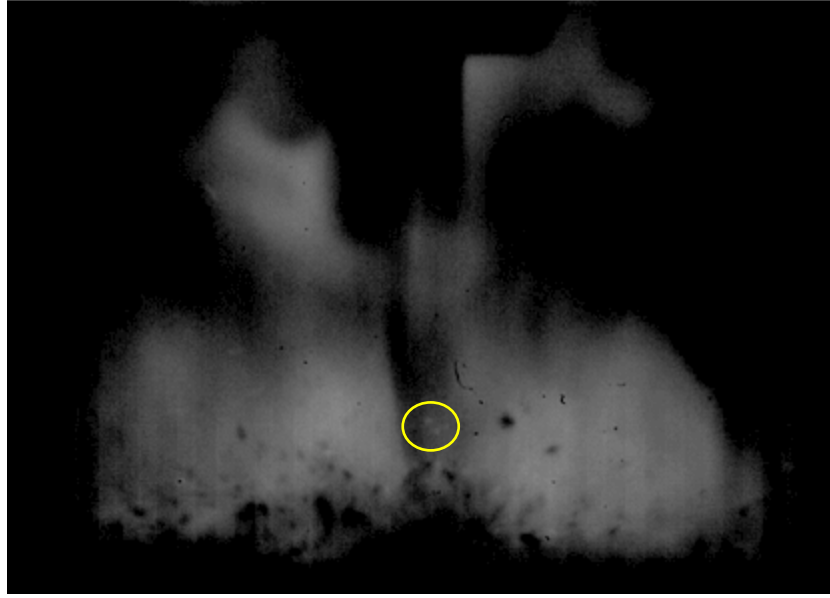
Fig. 11 Snapshot from the high-speed video of GO-coated nano-Al particles being ejected into the air 30 \mu s after being subjected to a 10.5-J discharge; the ejected particles appear black against the residual discharge emission since they are not burning, while a few smaller particles inside the yellow circle may be burning (picture has been cropped and the brightness/contrast adjusted)
