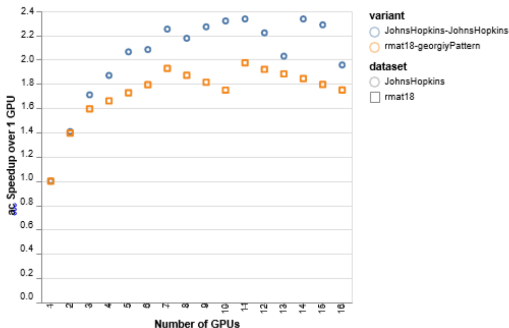
Scalability plots
