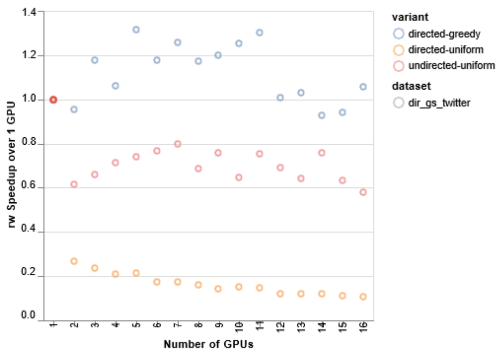
Scalability plots
