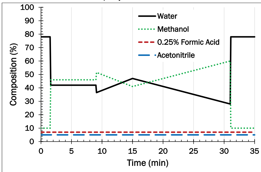
Figure 2. Graph showing gradient scheme for secondary method using Pinnacle II Biphenyl HPLC column.
