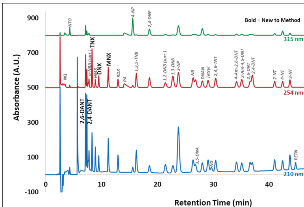
Figure 3. Chromatographic separation of 29 analytes and 2 surrogates using the reported primary method. Bolded analytes are new to the method; all other analytes and surrogates were previously reported under different separation conditions (Crouch et al. 2020). All analytes are at 5 mg/L in 50/50 methanol/water.
