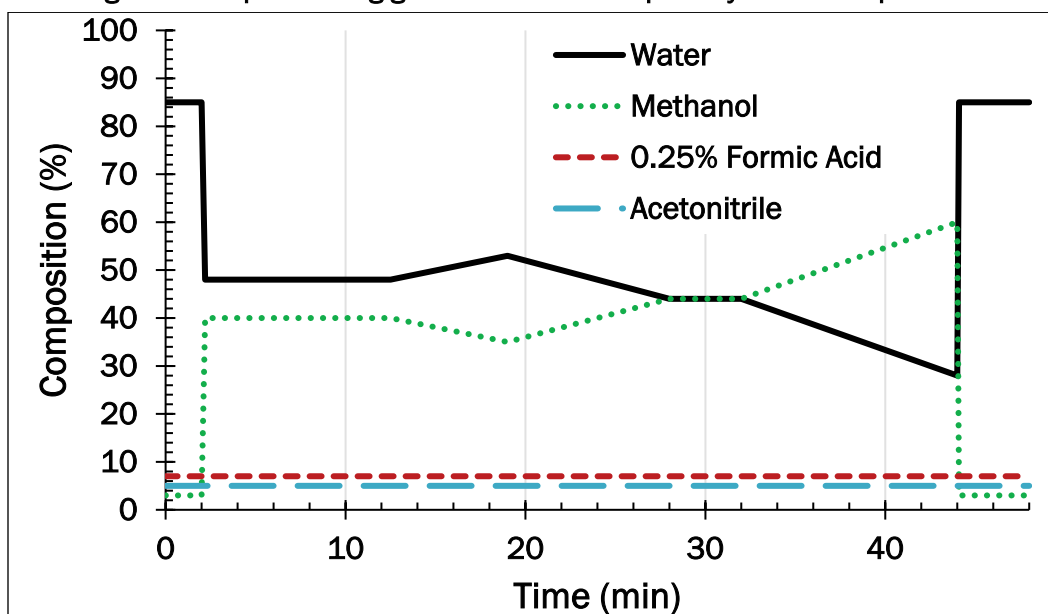
Figure 1. Graph showing gradient scheme for primary method separation.
