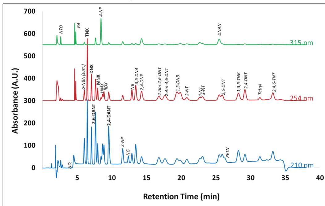
Figure 4. Secondary light chromatography–UV (LC–UV) method for separation of 29 munitions analytes and 2 surrogates by the reported secondary method. All analytes are at 5 mg/L in 50/50 methanol/water.
