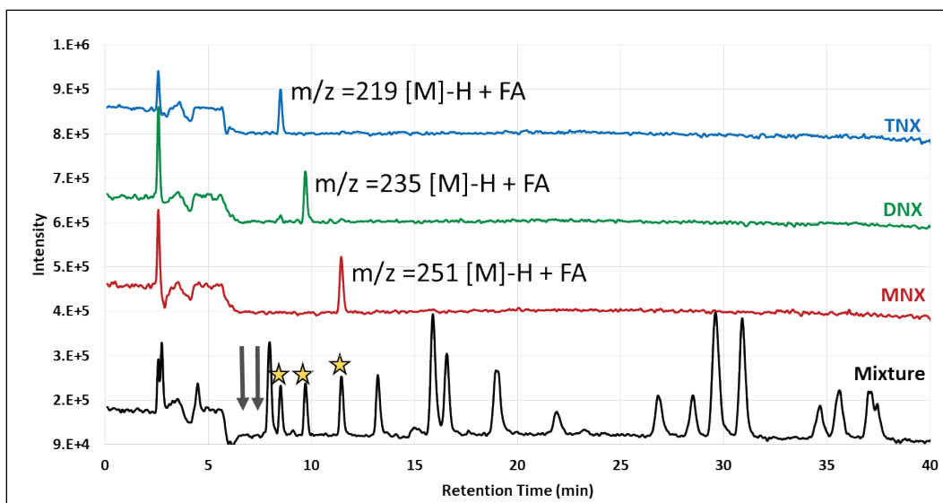
Figure 5. Mass spectrometric (MS) secondary method detection of MNX, DNX, and TNX in scan mode. Ion ( m/z ) peaks of MNX, DNX, and TNX are indicated with yellow stars. Arrows indicate where 2,6-DANT and 2,4-DANT elute but are not observed by the MS.
