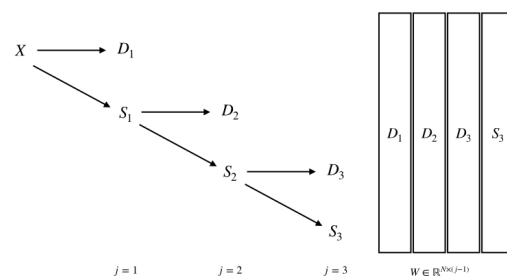
(b) Maximal Overlap Discrete Wavelet Transform (MODWT)
