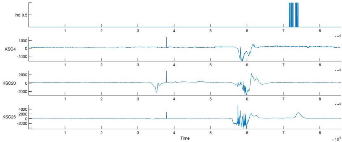
Figure 27: Top subplot is binary response of observed lightning, followed by three typical EFM measurements chosen randomly across the entire KSC/CCSFS region over time in seconds. The EFM measurements indicate a natural steady state in the absence of lightning, becoming increasingly chaotic as electromagnetic potential builds within the atmosphere.
