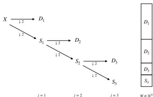
(a) Discrete Wavelet Transform (DWT)
