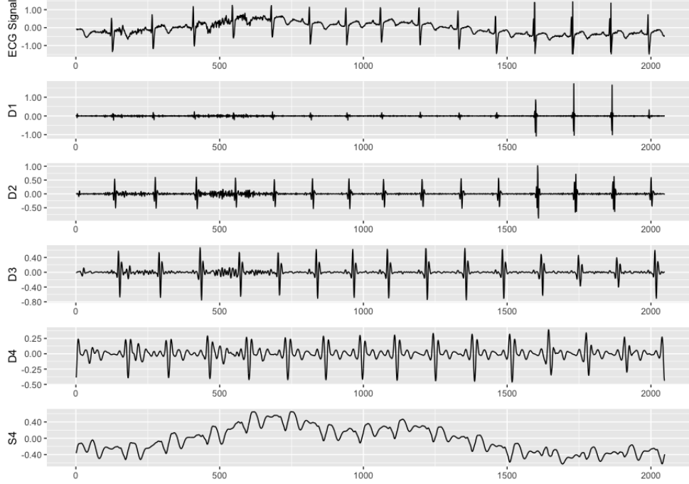
Figure 6: The shift invariant MODWT. Movement of coefficients align across resolution levels using four-level wavelet MRAs, utilizing the “la8” Daubechies wavelet filter, of an ECG signal as presented in Percival and Walden [73].
