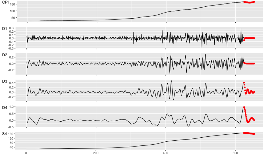
Figure 10: Forecast developed in the wavelet domain using the monthly U.S. consumer price index (CPI) from 1948 to 1999 dataset from the waveslim R package [95]. The original data is provided in the top subplot, with descending resolution levels of a four-level MODWT beneath. ARIMA models are fit each resolution level to produce thirty forecasted values (red), extending each individual resolution level. An inverse MODWT is applied to the extended resolution levels to a reconstructed CPI to include thirty forecasted values (red).
