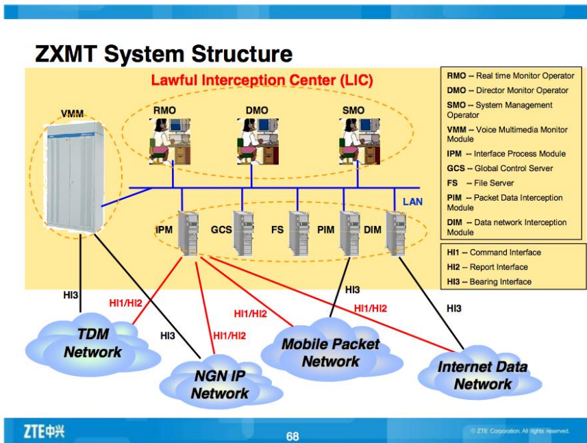
Figure 12. Page 68 of the ZTE marketing presentation shows the broad outlines of the system. It is likely that the images provided to Aikins include the data network interception module, labeled DIM here.
