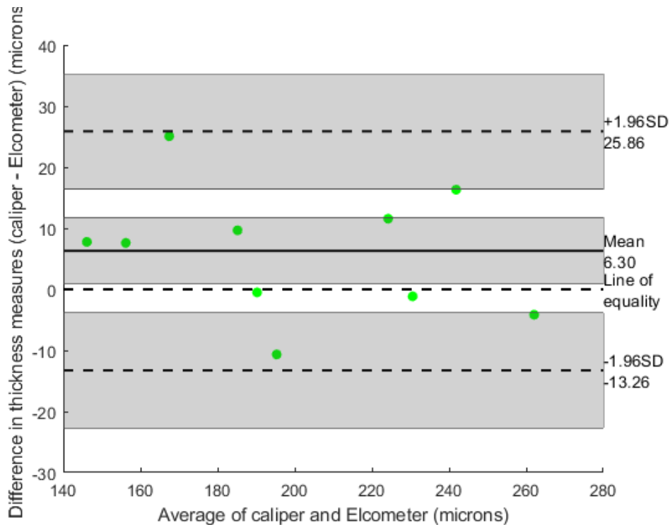
Fig. 5 Bland–Altman plot for thick samples (Elcometer-measured thickness greater than 105 \mu\text{m} )
