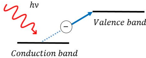
Figure 9. Excitation of an electron by a photon. The photoelectric effect is the basic operating principle for many types of detectors.
