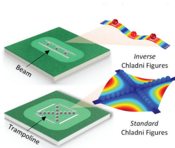
Figure 6.10: Doubly-clamped beams forming inverse Chladni Figures. Trampoline resonators forming standard Chladni Figures. Reprinted from Jia et al. , with the permission of AIP Publishing [16].
