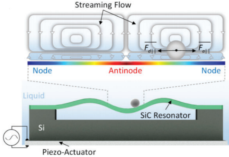
Figure 6.9: Schematic of microparticles showing forces resulting from mechanical vibration induced acceleration ( F_{a||} ), which point towards nodes, and forces resulting from streaming flows ( F_{d||} ), which point towards antinodes. Reprinted from Jia et al. , with the permission of AIP Publishing [16].
