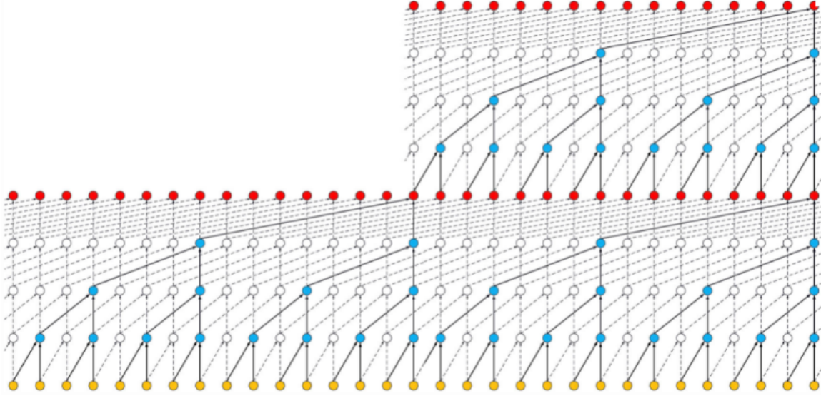
Figure 7. Visual illustration of a causal TCN with stacked blocks. This TCN has a block size of 2, a dilation list [1,2,4,8] (i.e. dilation factor 8), and a kernel size of 2 [68].
