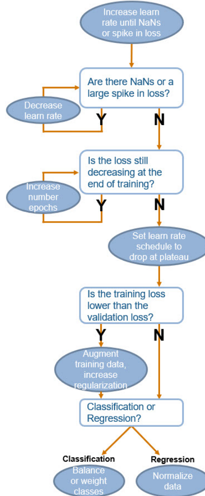
Figure 8. MATLAB Network Training Flowchart. Source [12].
