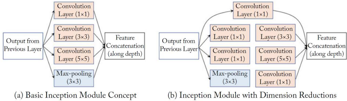
Figure 6. GoogLeNet Inception Module. Source [9].
