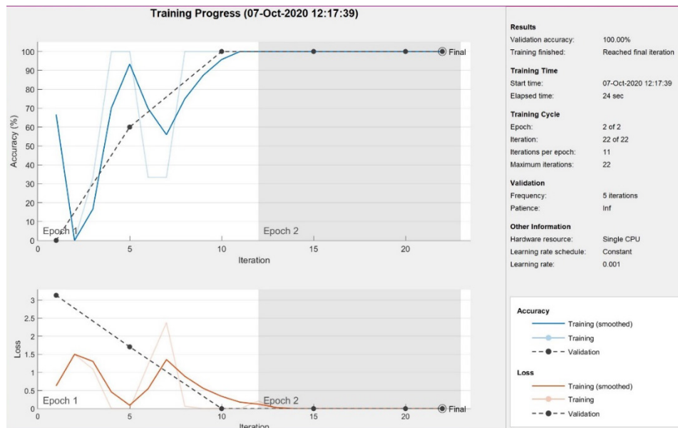
Figure 13. Training Progress Plot for Combined Image Network
