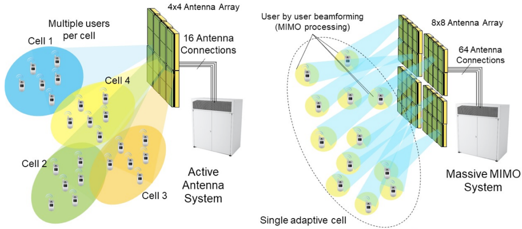
Figure 2.8. AAS vs massive MIMO. Source: [36].
