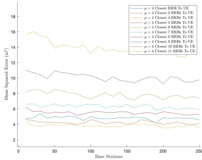
Figure A.7. The zoomed in view of mean square error for location error when \mu = 4 . The RRHs in the given area range from 3 to 250. Closest RRH to UE not in picture. Closest 3 RRHs to UE not pictured.
