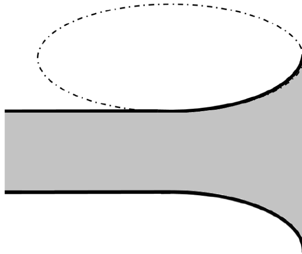
Figure 2. Elliptical profile bell mouth as described by Wallen. Source: [4].
