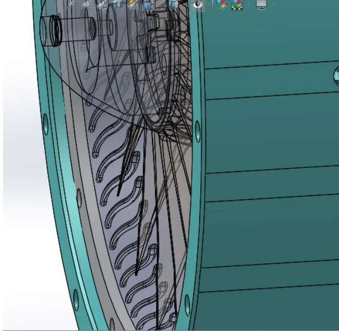
Figure 17. SolidWorks Representation of S-Grooves Cast into Epoxy Layer
