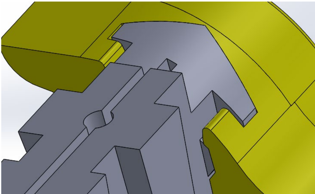
Figure 19. S-Mold Base and Top Connection
