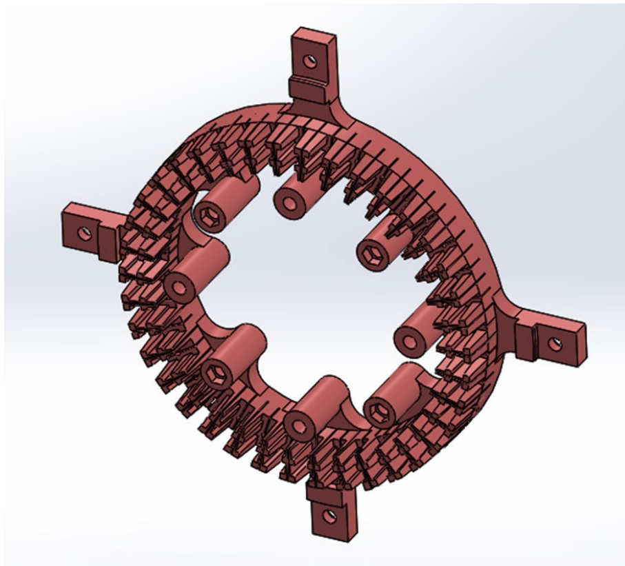
Figure 12. Main Disk SolidWorks Model
