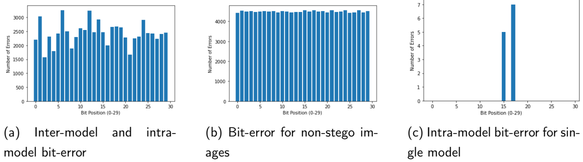
Figure 4.16. Comparison of relative bit-error position across multiple models (a), against cover images only (b), and within a single epoch/model (c).
