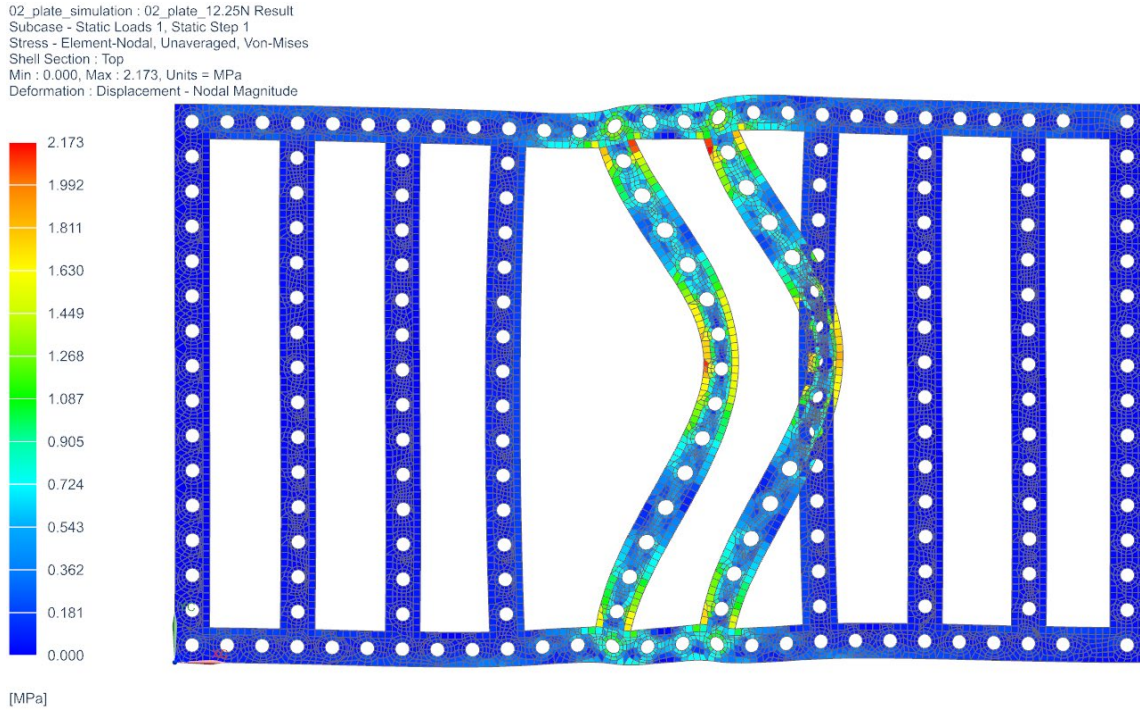
Figure 9. Stress results with 12.25 N load on center rails—plate pinned on the four corners
