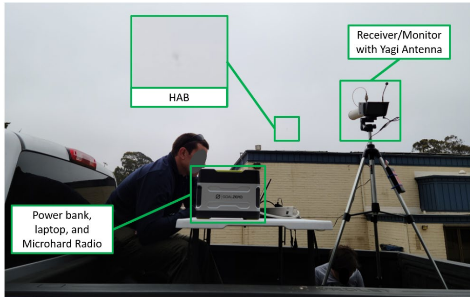
Figure 46. Mobile ground segment
