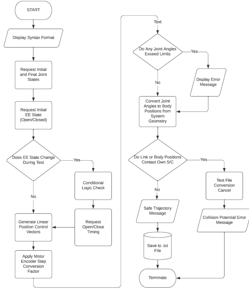
Figure 20. Trajectory Generation Program Workflow
