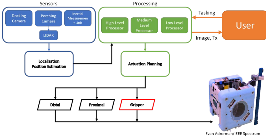
Figure 7. Astrobee Robotic System Block Diagram. Adapted from [17], [18]
