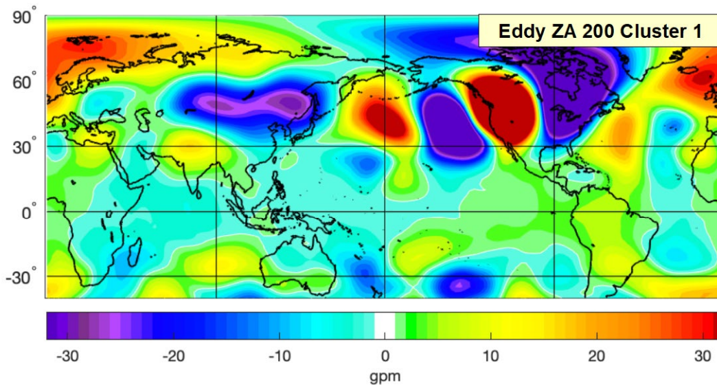
Figure 35. Composite 200 mb eddy geopotential height anomaly (gpm) for the days in cluster 1 of the November CA 850 mb u and v winds.
