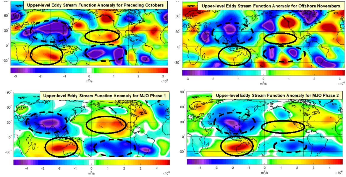
Figure 24. Upper-level eddy stream function anomaly ( \text{m}^2/\text{s} ) one (top left) and zero-months (top right) prior to the top 15 offshore Novembers compared to upper-level eddy stream function anomaly ( \text{m}^2/\text{s} ) for Oct–Nov MJO phases 1 (bottom left) and 2 (bottom right).
