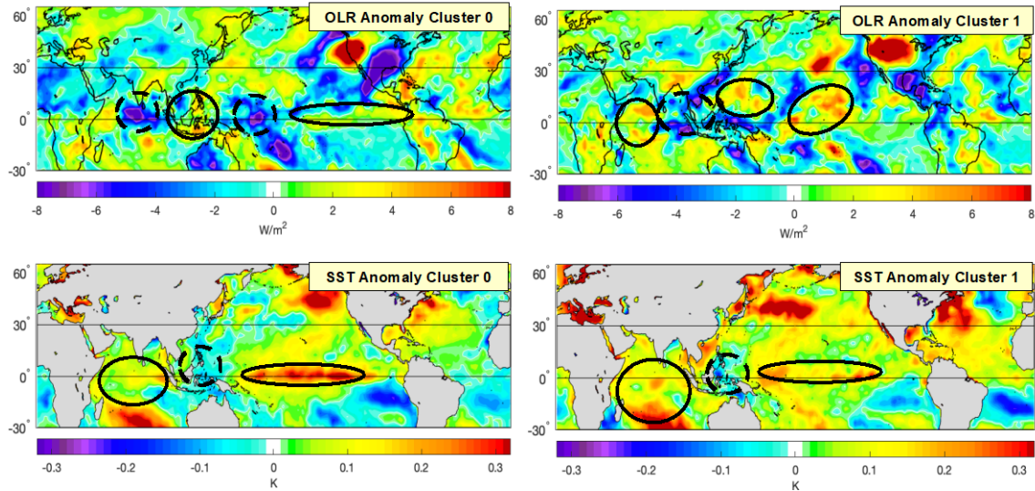
(Top) Solid (dashed) black circles represent positive (negative) OLR anomalies. (Bottom) Solid (dashed) black circles represent positive (negative) SST anomalies.
