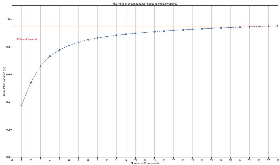
Figure 45. Cumulative PCA variance by number of components.
