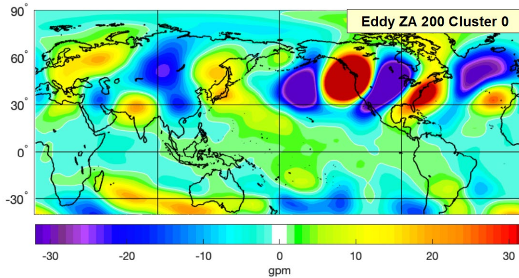
Figure 34. Composite 200 mb eddy geopotential height anomaly (gpm) for the days in cluster 0 of the November CA 850 mb u and v winds.
