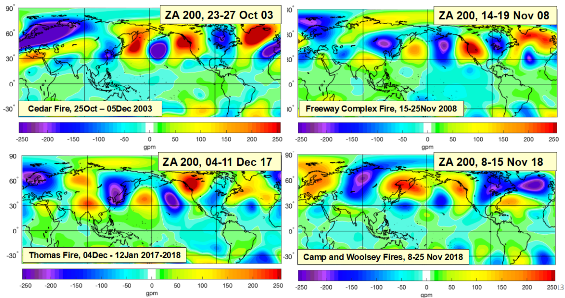
Figure 8. Global view of the 200 mb eddy geopotential height (gpm) anomalies and associated wildfires for four CA OWEs.
