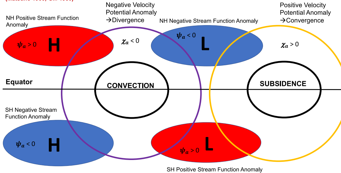
Figure 62. Schematic detailing how to infer upper-level stream function and velocity potential anomalies from tropical convective anomalies.
