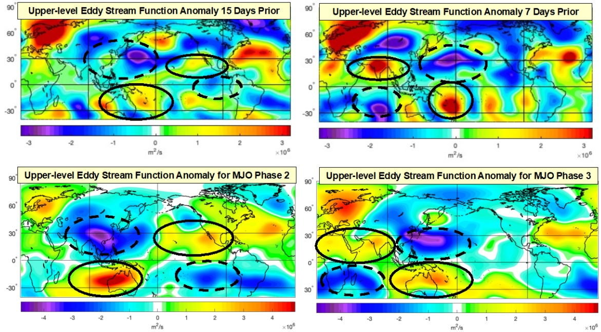
OWE eddy stream function anomaly plots (top row) are comprised of nine-day means centered on 15 and seven days prior to CA OWE events. MJO phase composites (bottom row) represent the composite eddy stream function anomaly for MJO phase 2 and 3 events in Oct–Nov 1979–2018.
