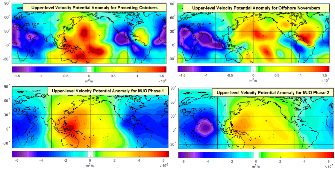
Figure 26. Upper-level velocity potential anomaly ( \text{m}^2/\text{s} ) one (top left) and zero-months (top right) prior to the top 15 offshore Novembers compared to upper-level velocity potential anomaly ( \text{m}^2/\text{s} ) for Oct–Nov MJO phases 1 (bottom left) and 2 (bottom right).
