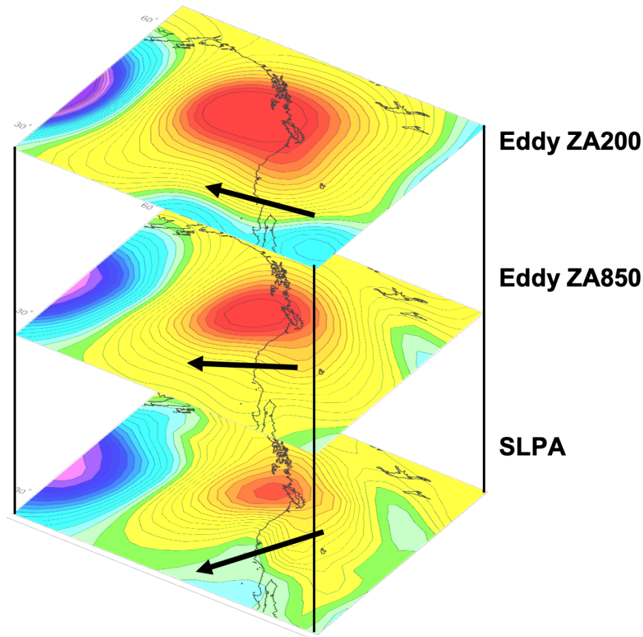
Eddy geopotential height anomaly (gpm) for the upper (200 mb) and lower (850 mb) troposphere and sea level pressure anomaly plots for the 23–27 October 2003 Santa Ana event.
