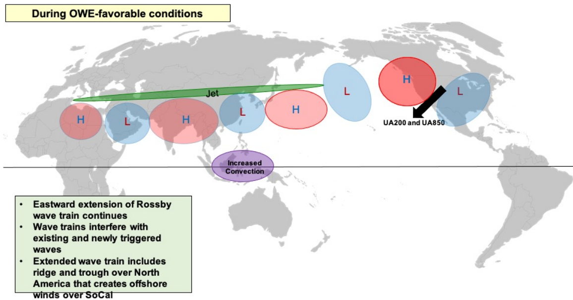
Figure 44. Conceptual schematic of hypothesized teleconnection dynamics just prior to and/or during CA OWEs.
