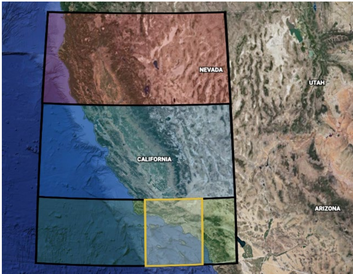
The large black box encompassing California represents the All-CA focus region. The individual red, blue and green shaded boxes encompass the Northern, Central and Southern CA subregions, respectively. The yellow outlined box encompasses the SA subregion.
