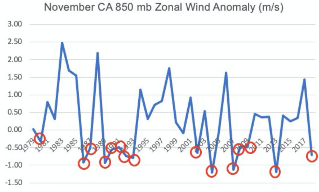
Monthly mean November CA 850 mb zonal wind anomaly. The red circles identify the 15 most offshore favorable Novembers, in terms of monthly mean wind speed anomalies.
