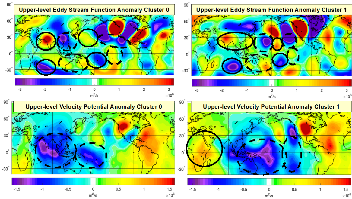
(Top) Solid (dashed) black circles represent anticyclonic (cyclonic) circulations. (Bottom) Solid (dashed) black circles represent upper-level convergent wind (divergent wind).
