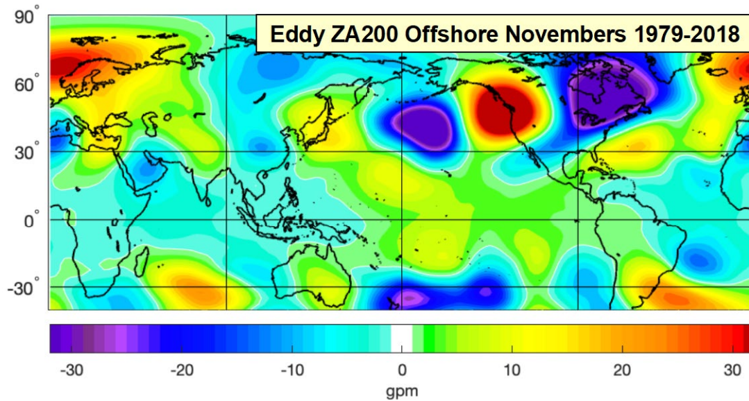
Figure 20. November monthly mean 200 mb eddy geopotential height anomaly (gpm) composite for the 15 most offshore Novembers, 1979–2018.
