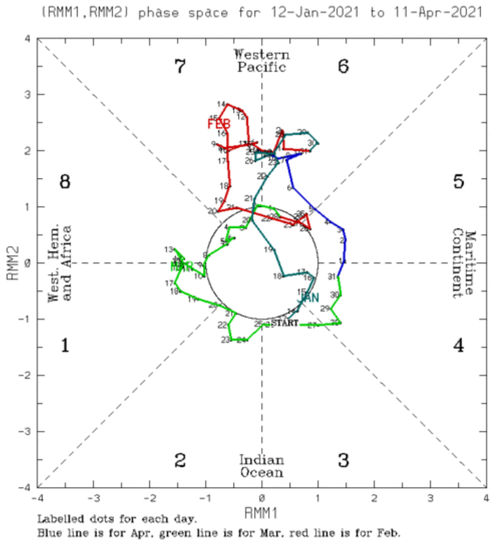
Figure 17. Sample MJO phase diagram. Source: BOM (2021).
