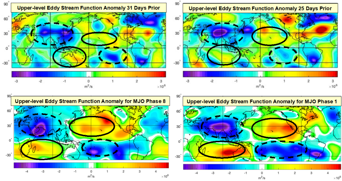
OWE eddy stream function anomaly plots (top row) are comprised of nine-day means centered on 31 and 25 days prior to CA OWE events. MJO phase composites (bottom row) represent the composite eddy stream function anomaly for MJO phase 8 and 1 events in Oct–Nov 1979–2018.
