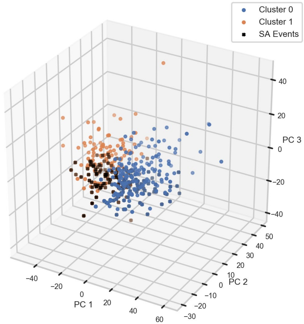
Figure 49. 3D plot of CA OWE events in PC space.
