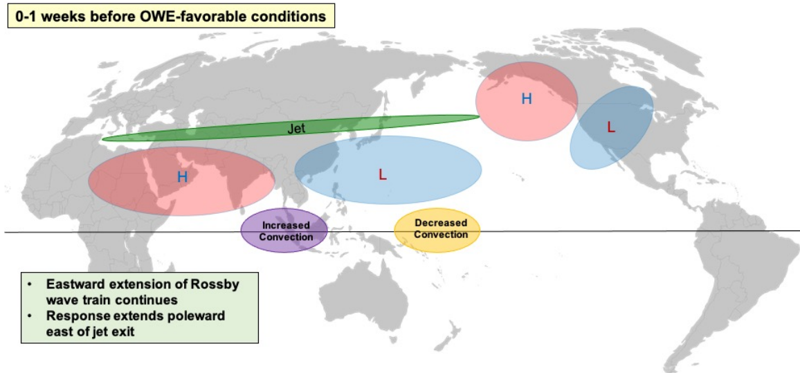
Figure 43. Conceptual schematic of hypothesized teleconnection dynamics zero to one weeks before CA OWEs.
