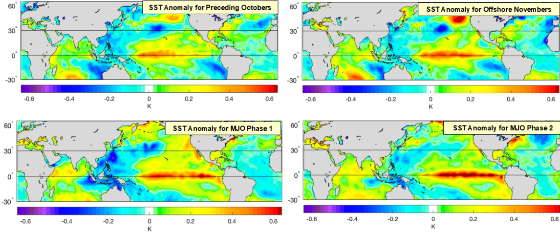
Figure 28. SST anomalies (C) one (top left) and zero-months (top right) prior to the top 15 offshore Novembers compared to SST anomalies (C) for Oct–Nov MJO phases 1 (bottom left) and 2 (bottom right).
