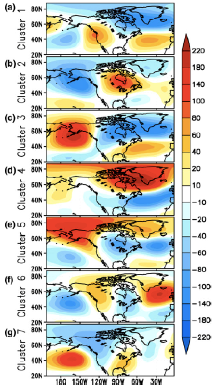
K-mean cluster composites of North American 500 mb geopotential heights anomalies (seven-day means) for seven clusters (a–g).
