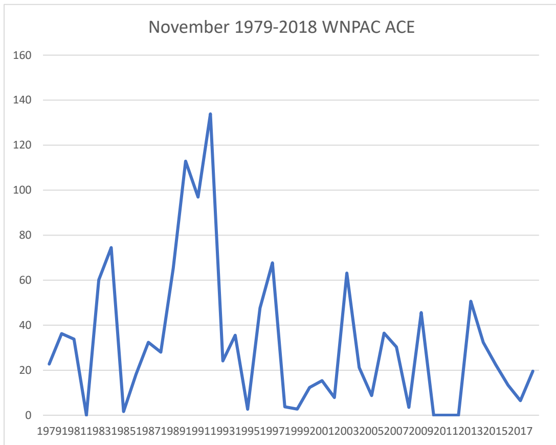
Figure 16. Monthly mean ACE for the NWPAC for November 1979–2018.
