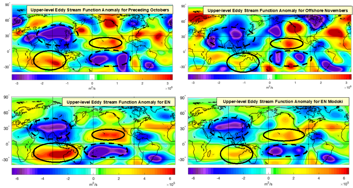
Figure 25. Upper-level sigma eddy stream function anomaly ( \text{m}^2/\text{s} ) one (top left) and zero-months (top right) prior to the top 15 offshore Novembers compared to upper-level sigma eddy stream function anomaly ( \text{m}^2/\text{s} ) for Oct–Nov EN (bottom left) and EN Modoki (bottom right).
