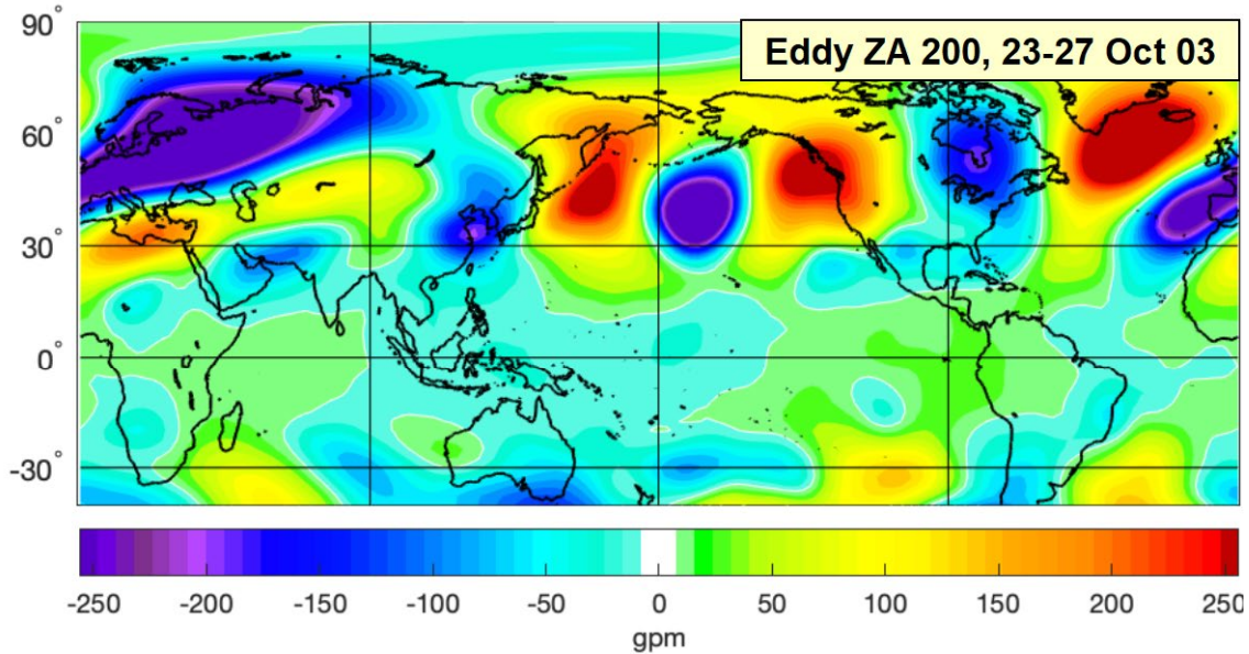
Figure 7. Global view of the 200 mb eddy geopotential height (gpm) anomaly for the October 23–27, 2003 OWE.
