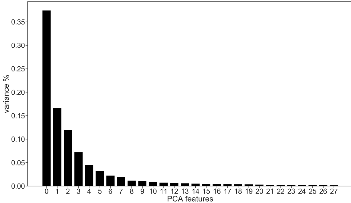
Figure 46. Percent Variance explained by each PCA component
