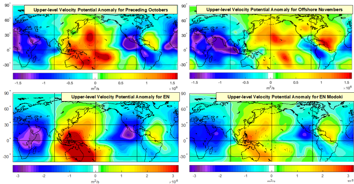
Figure 27. Upper-level velocity potential ( \text{m}^2/\text{s} ) one (top left) and zero-months (top right) prior to the top 15 offshore Novembers compared to upper-level velocity potential anomaly ( \text{m}^2/\text{s} ) for Oct–Nov EN (bottom left) and EN Modoki (bottom right).
