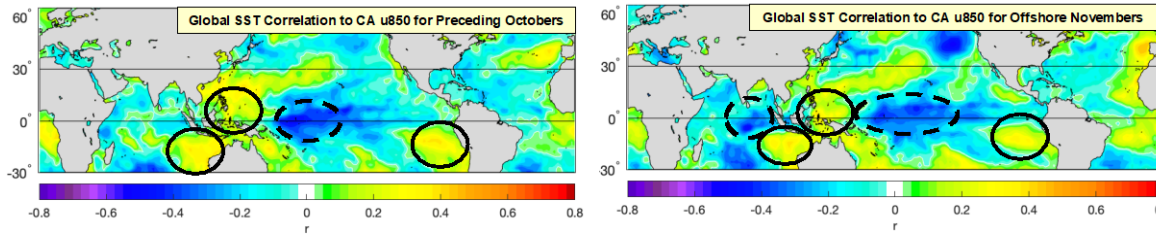
Figure 31. Correlations for CA November 850 mb zonal wind to global SST one (left) and zero-months (right) prior to the top 15 offshore Novembers.
