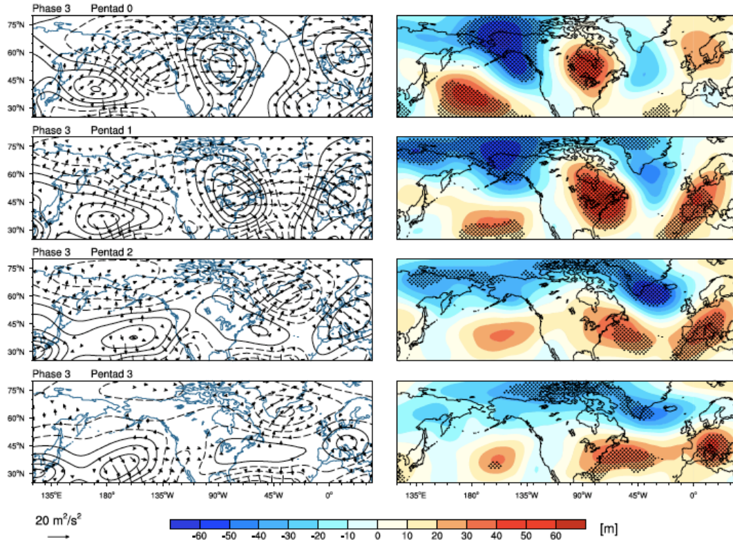
Anomalous upper-level stream function (left) zero to three pentads after MJO Phase 3. Black arrows represent wave activity flux vectors. Anomalous 500 mb geopotential heights (right) zero to three pentads after MJO Phase 3. Black dots represent statistically significant anomalies.
