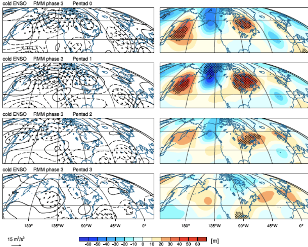
Figure 12. Prior research investigating stream function and geopotential heights over WNA lagging MJO Phase 3 by zero to 15 days, during LN conditions. Adapted from Henderson and Maloney (2018).
