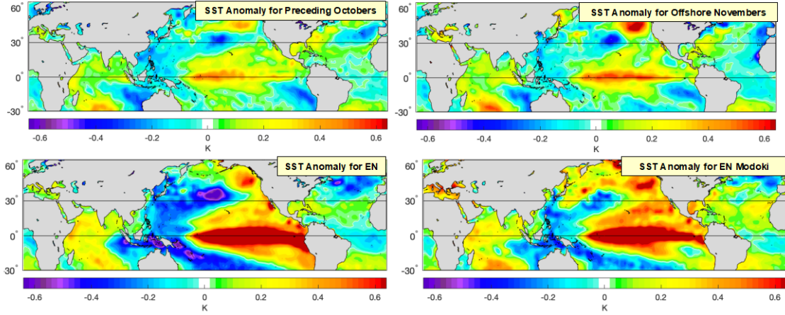
Figure 29. SST anomalies (C) one (top left) and zero-months (top right) prior to the top 15 offshore Novembers compared to SST anomalies (C) for Oct–Nov EN (bottom left) and EN Modoki (bottom right).
