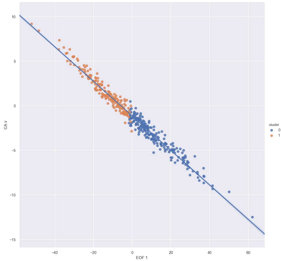
Figure 52. Scatter plot of CA v wind speed vs. EOF (PC) 1
