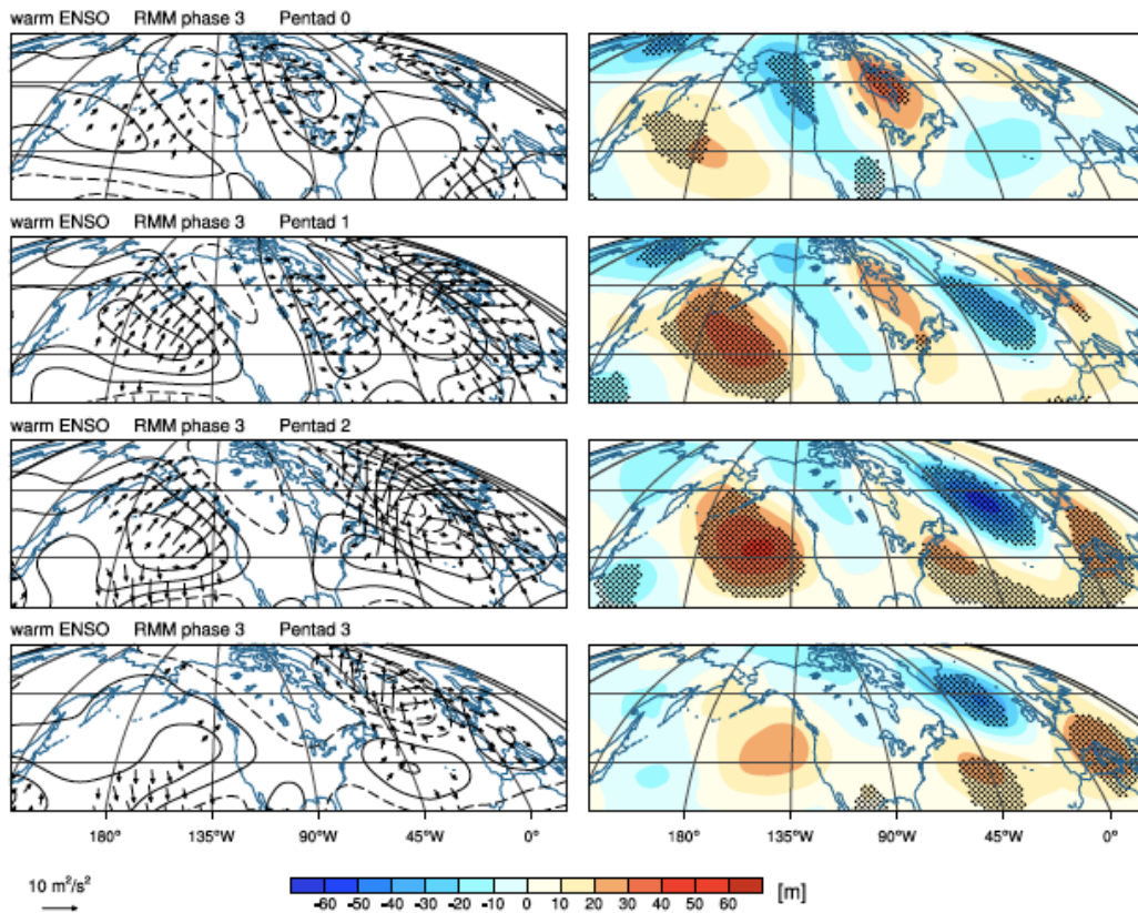
Figure 11. Prior research investigating stream function and geopotential heights over WNA lagging MJO Phase 3 by zero to 15 days, during EN conditions. Adapted from Henderson and Maloney (2018).
