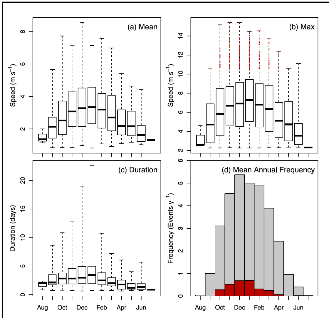
Climatology of SA events from 1948 to 2021: a) monthly distribution of SA event mean wind speed, b) monthly distribution of SA event max wind speed, c) monthly distribution of SA event duration, and d) mean monthly SA event frequency. Extreme events of > 10–15 \text{m s}^{-1} are noted in red.
