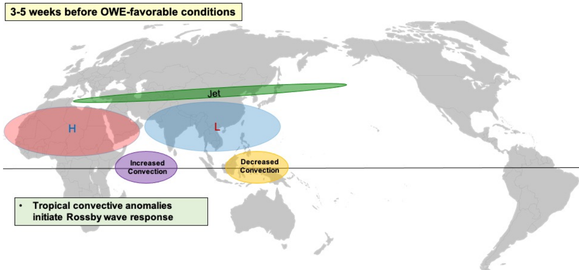
Figure 41. Conceptual schematic of hypothesized teleconnection dynamics three to five weeks before CA OWEs.
