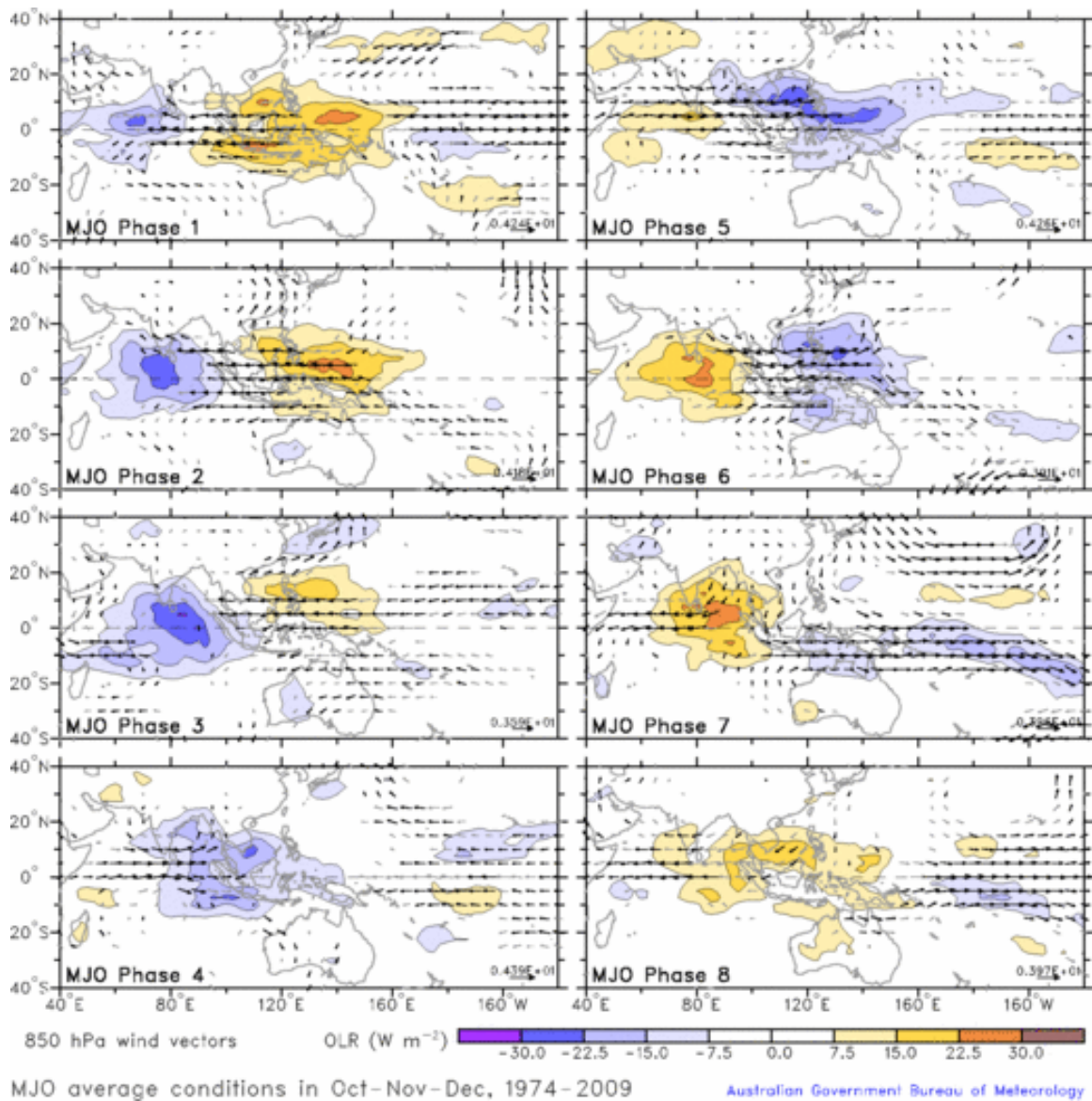
Figure 18. Average OLR and 850 mb wind patterns per phase for October to December 1974–2009.
