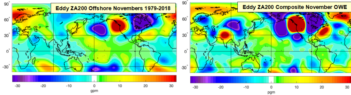
Figure 21. Comparison of November monthly mean 200 mb eddy geopotential height anomaly (gpm) composite for the 15 most offshore months (left) and eddy geopotential height anomaly (gpm) composite of the 200 most offshore individual November days (right).
