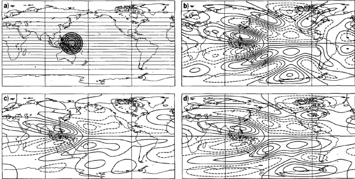
(a) Idealized stream function and divergence perturbation (shaded). The anomalous stream function evolution 48-days later is portrayed using a linear (b), partially nonlinear (c), and fully nonlinear (d) model.
