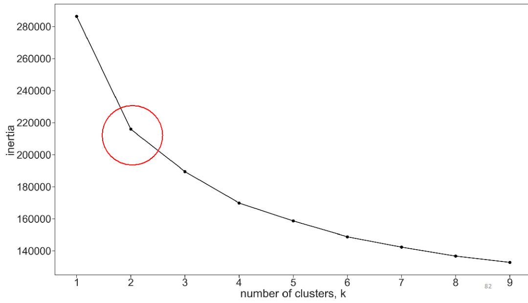
Figure 47. Inertia Score for k clusters.
