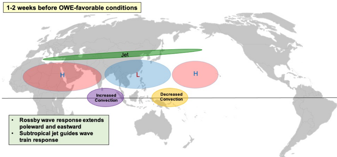
Figure 42. Conceptual schematic of hypothesized teleconnection dynamics one to two weeks before CA OWEs.
