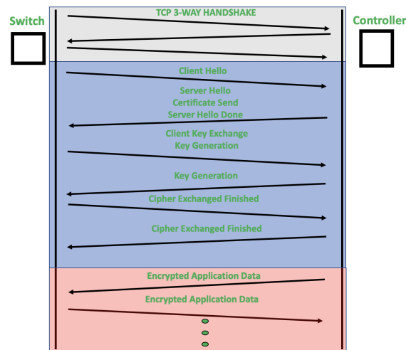
Figure 2.3. TLS 1.2 Connection Establishment
