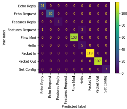
(a) Decision Tree Confusion Matrix
