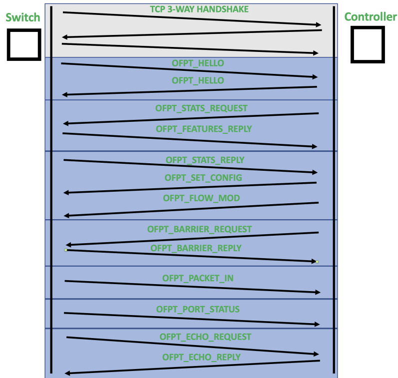
Figure 3.2. OpenFlow Message Diagram
