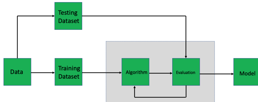
Figure 3.11. Classification Algorithm Development
