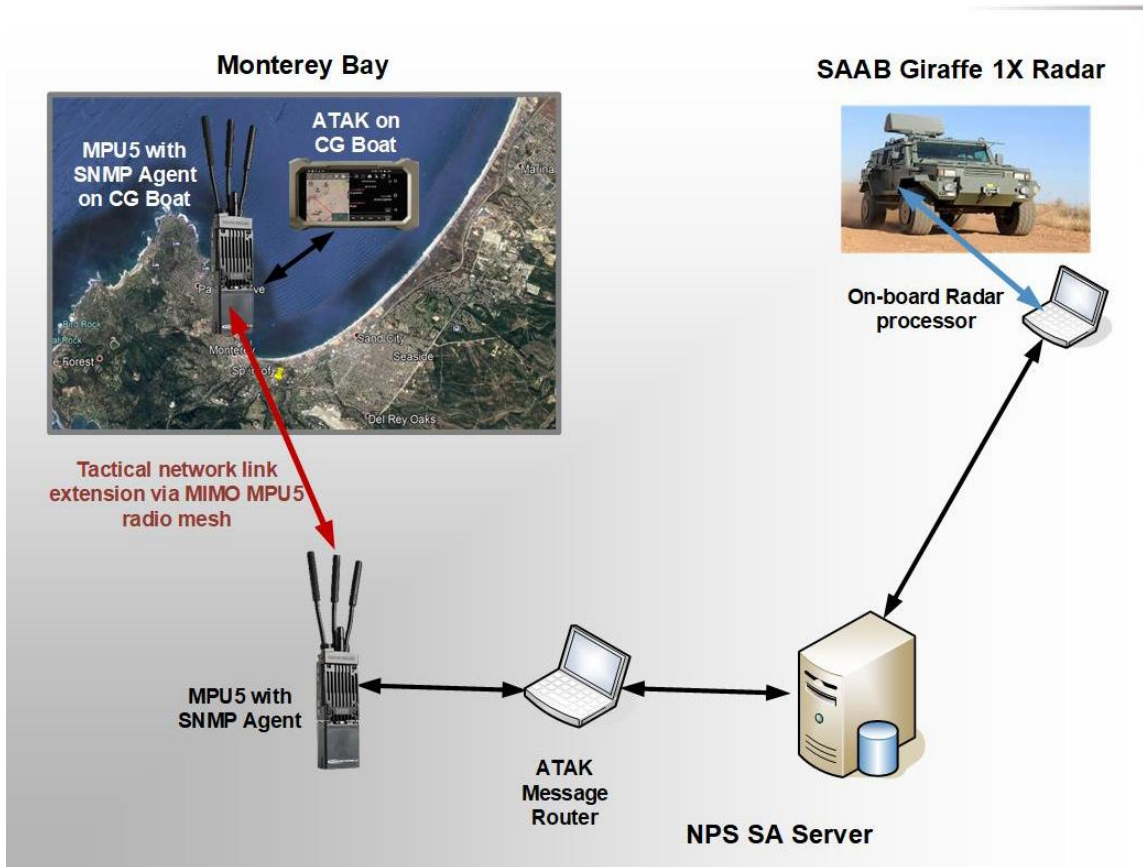
Figure 20. Overview of Phase 4 Network
