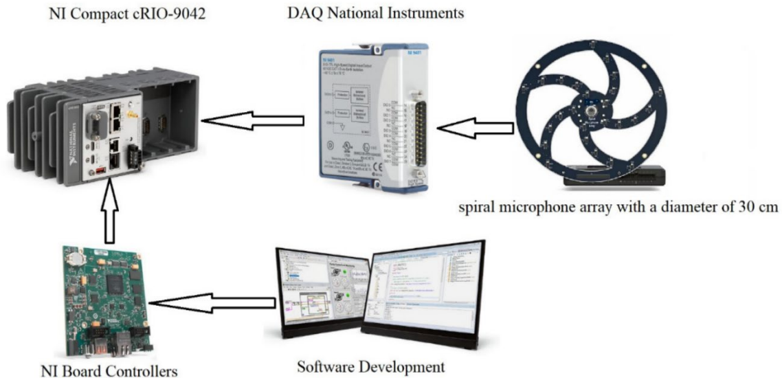
Figure 6. Acoustic System for UAS Detection. Source: Dumitresu et. al. (2020).
