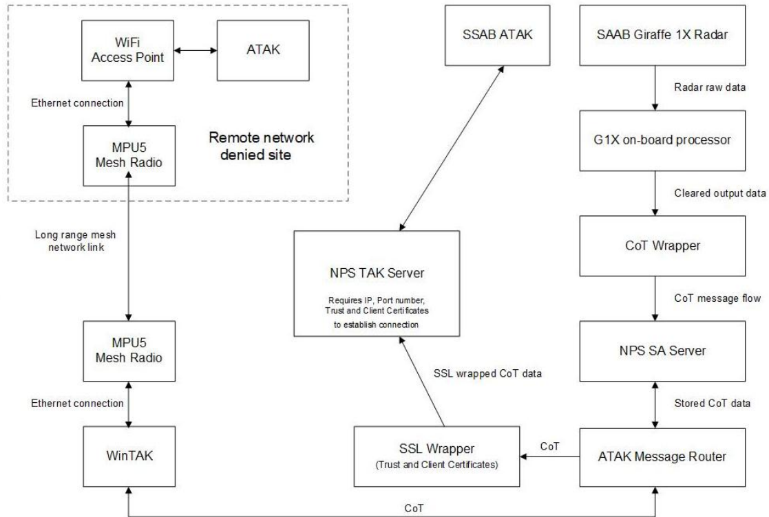
Figure 17. Network Diagram of Phase 4
