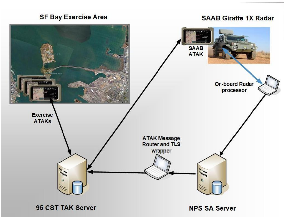
Figure 16. Overview of Phase 3 Network
