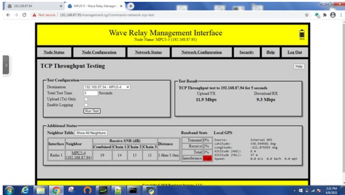
Figure 29. Actual TCP Throughput for WMN Extension, During Experimentation
