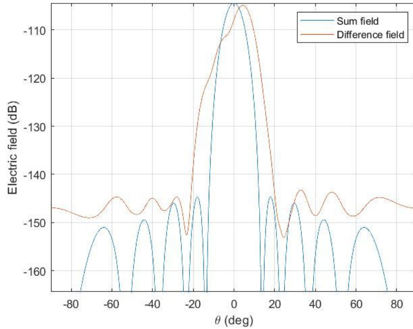
Figure 13. Received sum and difference beams of the target and jammer
