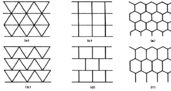
Figure 7. Packing of two-dimensional cells to fill a plane. Source: [12].
