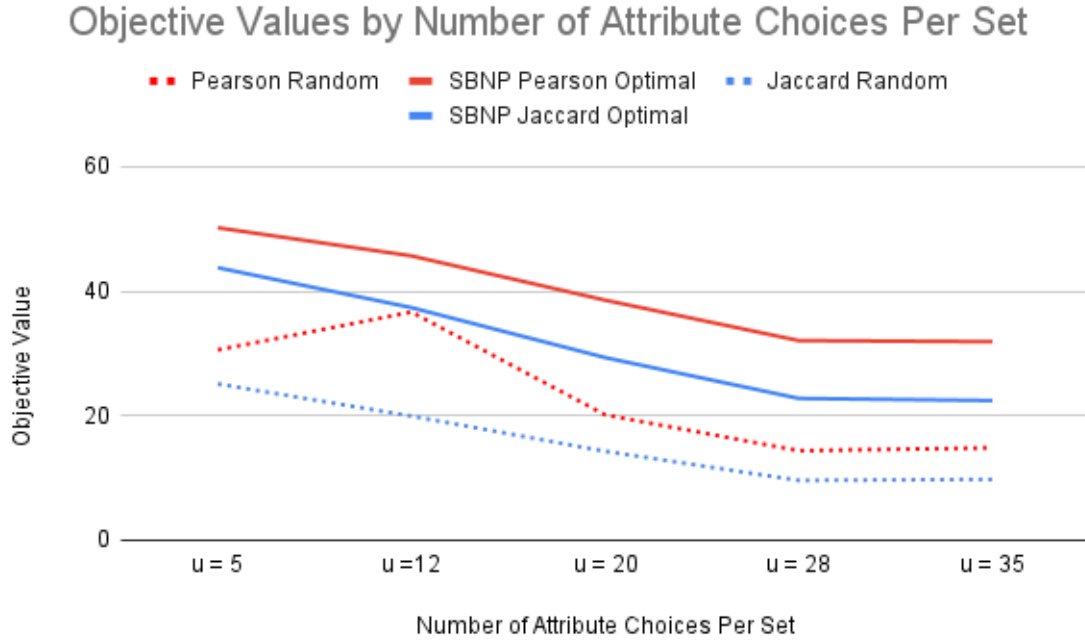
Figure 4.4. Number of Choices Per Attribute Set Comparison: The relationship between each method's objective value is compared across each number_of_choices_per_attribute_set value.
