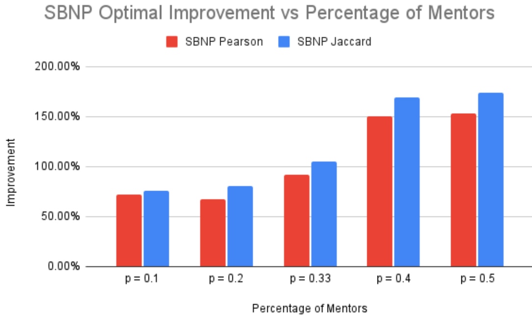
Figure 4.6. Percentage of Mentors Similarity Metric Analysis: The percentage of improvement for each similarity metric's performance is compared across different percentage_of_mentors values.
