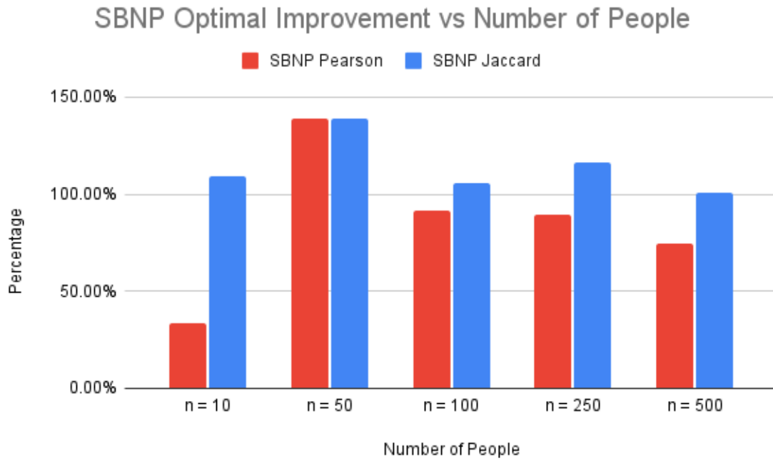
Figure 4.5. Number of People Similarity Metric Analysis: The percentage of improvement for each similarity metric's performance is compared across different number_of_people values.
