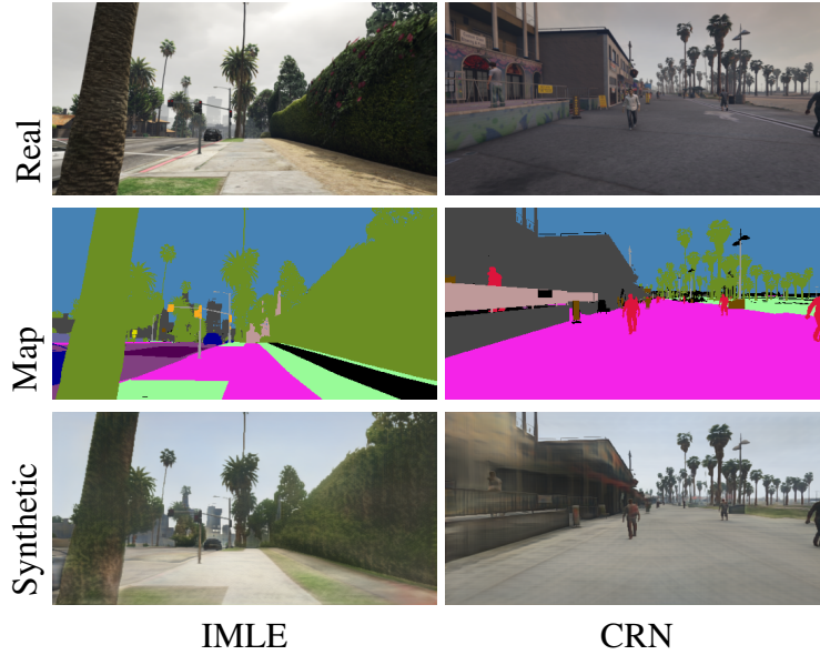
Figure 2.9. Representative images from the non-adversarial semantic layout datasets. A semantic layout map is included in the middle row for context. Wang et al. (2020) use only the real and synthetic images to test their classifiers. Real and synthetic images from Wang et al. (2020) Git repository and derived from Li et al. (2019); Chen and Koltun (2017). Semantic maps sourced directly from Li et al. (2019).
