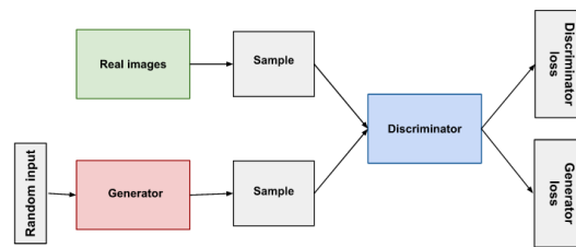
Figure 2.4. An illustration of a simple GAN architecture. A discriminator is initially trained on real images, while a generator initializes with random inputs. Generated data is passed to the discriminator, whose classification outputs influence both generator and discriminator loss. Source: Google Developers (2019).
