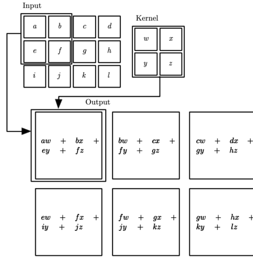
Figure 2.3. An illustration of a single CNN convolution. A 2x2 kernel operates on a 3x4 array with stride 1 (i.e., slides one unit at a time), producing a 2x3 output. Source: Goodfellow et al. (2016).
