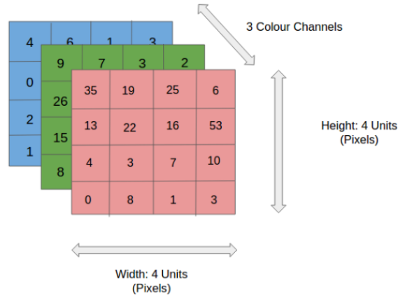
Figure 2.2. An illustration of an RGB image tensor. Color information for the image is spread across three individual arrays. Source: Saha (2018).
