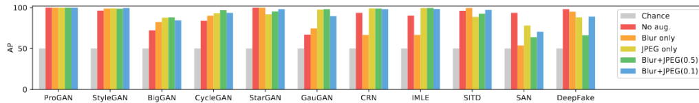
Figure 3.1. AP performance by dataset and model in the original analytic. Source: Wang et al. (2020).
