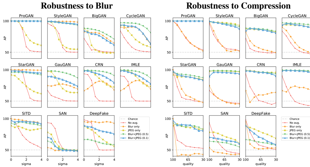
Figure 3.2. AP performance by dataset and model against test images augmented with blur and compression. Source: Wang et al. (2020).
