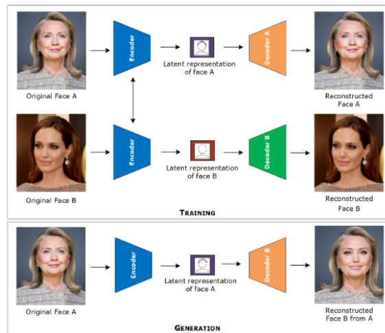
Figure 2.5. An illustration of the encoder/decoder training process and the creation of a deepfake. Note that the target face is passed to the source's decoder for reconstruction. Source: Masood et al. (2021).
