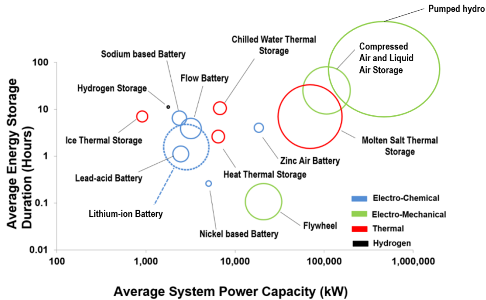
Figure 1. Energy Storage Technologies. Adapted from Fu, Remo, and Margolis (2018).
