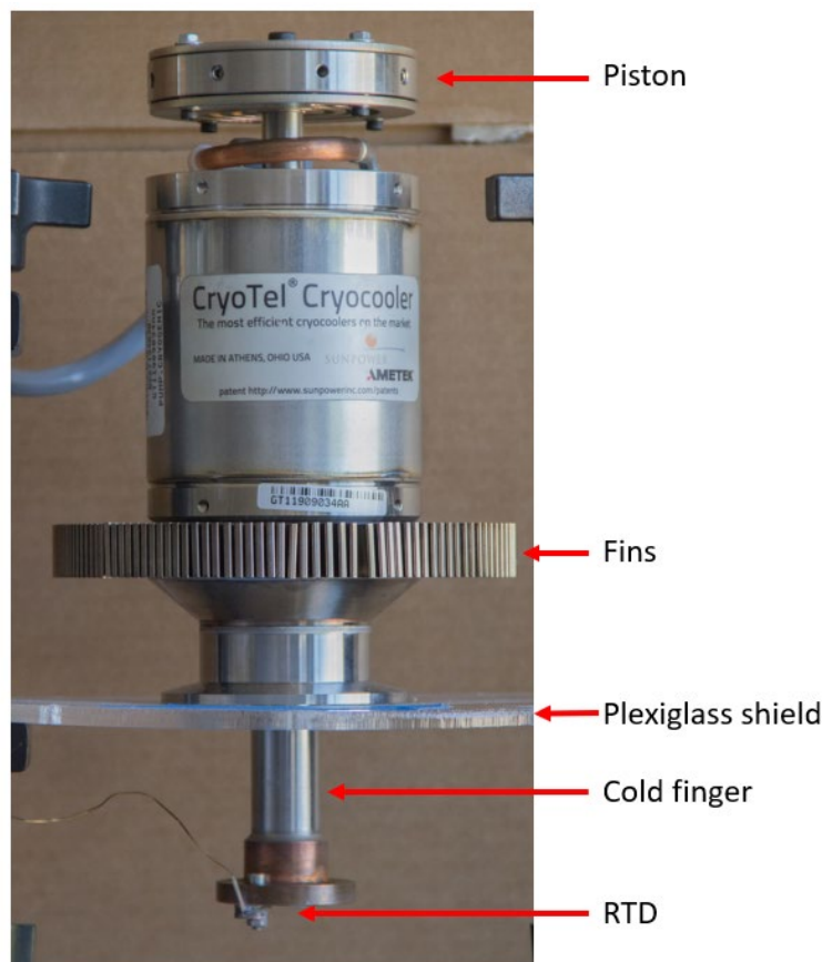
Figure 8. CryoTel GT Cryocooler
