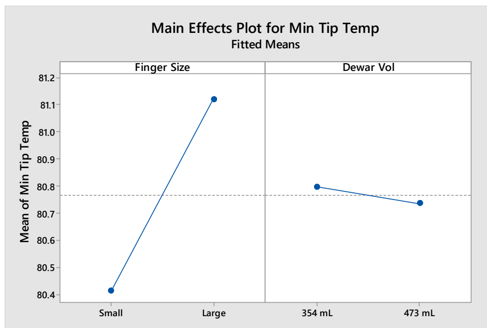
Figure 24. Main Effects Plot for the Minimum Tip Temperature
