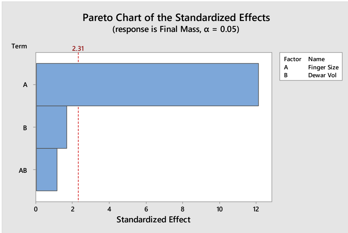
Figure 19. Final Production Mass Pareto Chart
