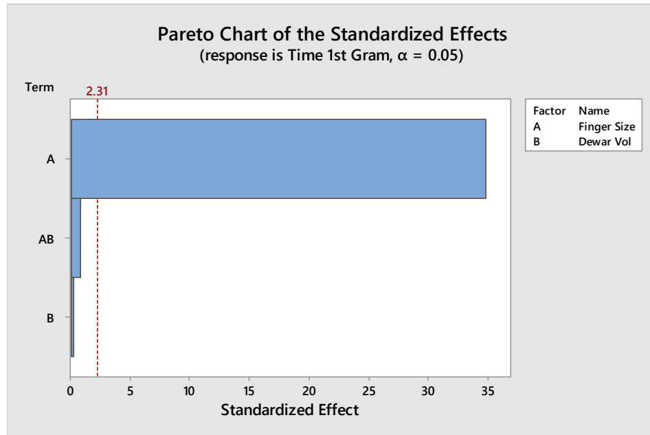
Figure 21. Time to First Gram Pareto Chart
