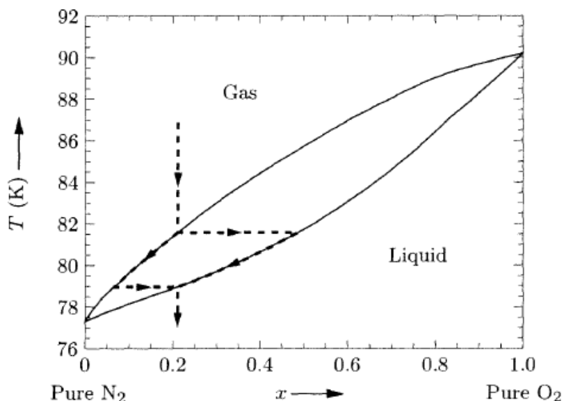
Figure 7. Phase Diagram for Atmospheric Air. Source: Schroeder (2000).
