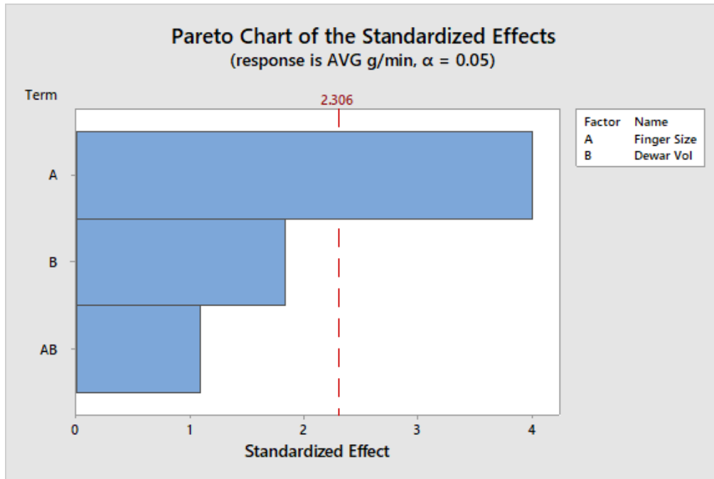
Figure 17. Average Production Pareto Chart
