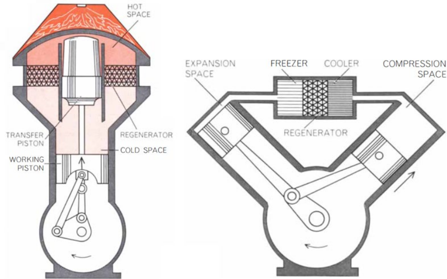
Figure 5. Two Stirling Engine Configurations. Source: Kohler (1965).
