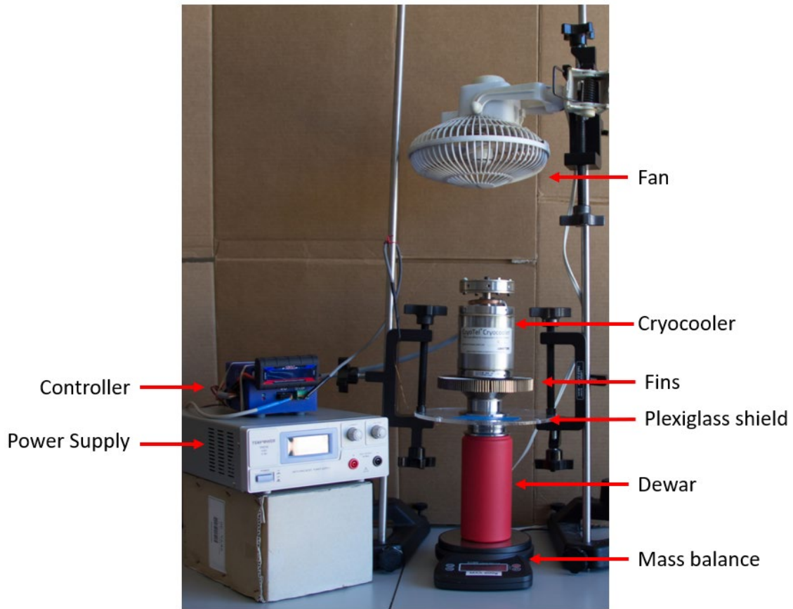
Figure 15. Experimentation Setup
