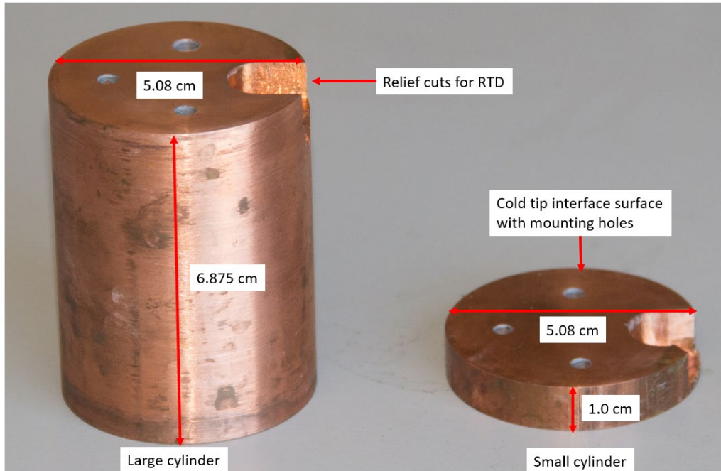
Figure 9. Cold Finger Extension
