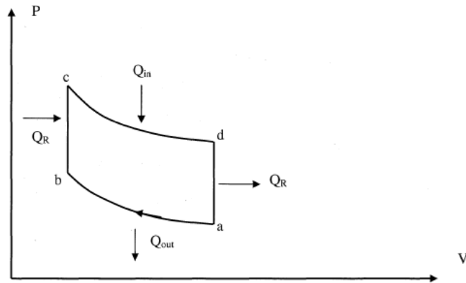
Figure 4. Stirling Cycle PV Diagram. Source: Shaw (2008).
