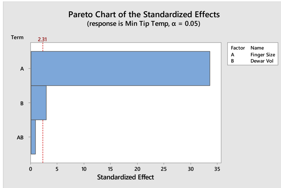
Figure 23. Minimum Tip Temperature Pareto Chart
