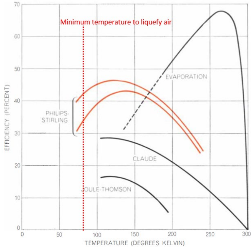
Figure 6. Cooling Efficiencies. Adapted from Kohler (1965).
