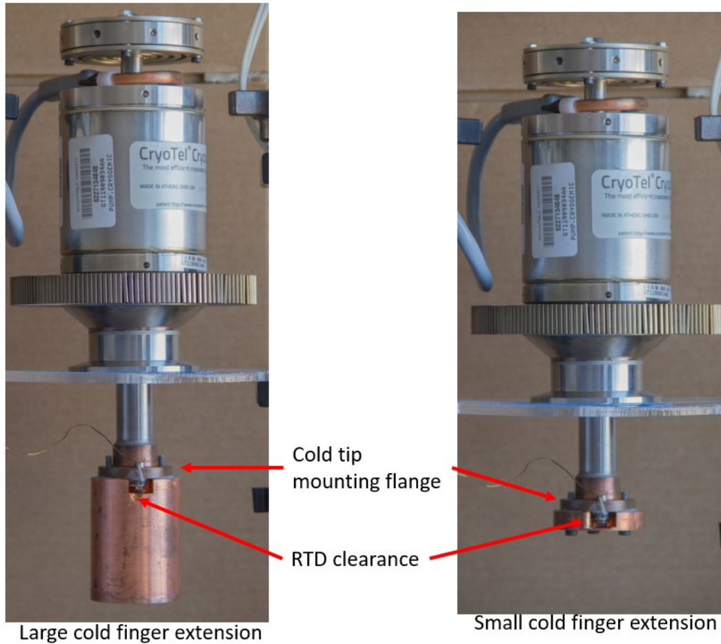
Figure 10. Cold Finger Extensions Mounted on Cryocooler
