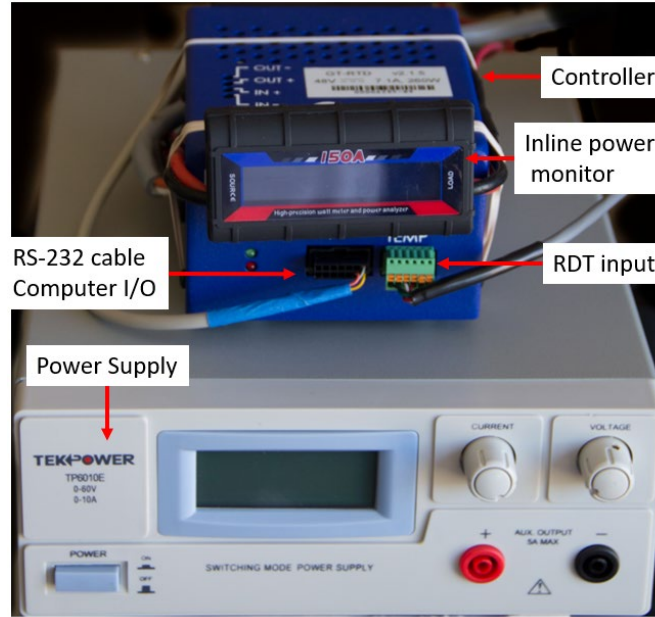
Figure 16. Electronics Setup
