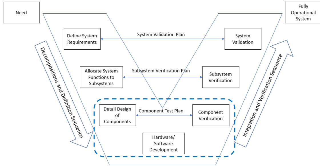
Figure 2. Systems Engineering V-Model. Adapted from Forsberg and Mooz (1992).
