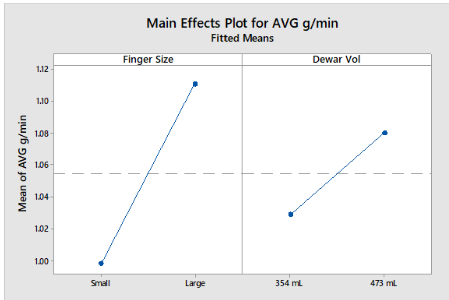
Figure 18. Main Effects Plot for Average Production Rate
