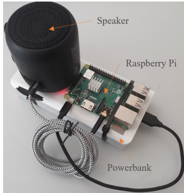
Figure 35. Mobile Hit Actor Hardware Setup
